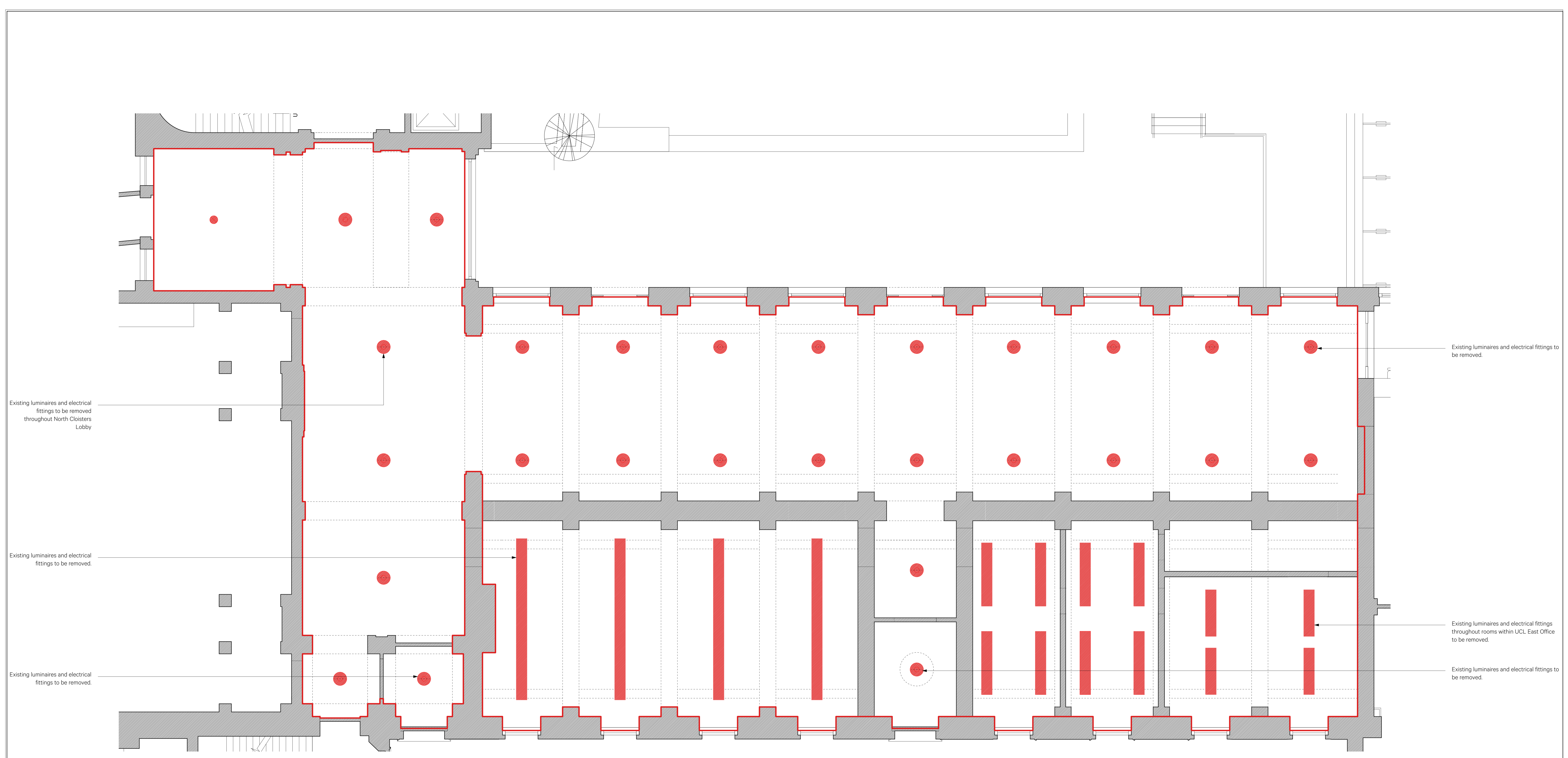
1 North Cloisters Demolition RCP 150@A0
