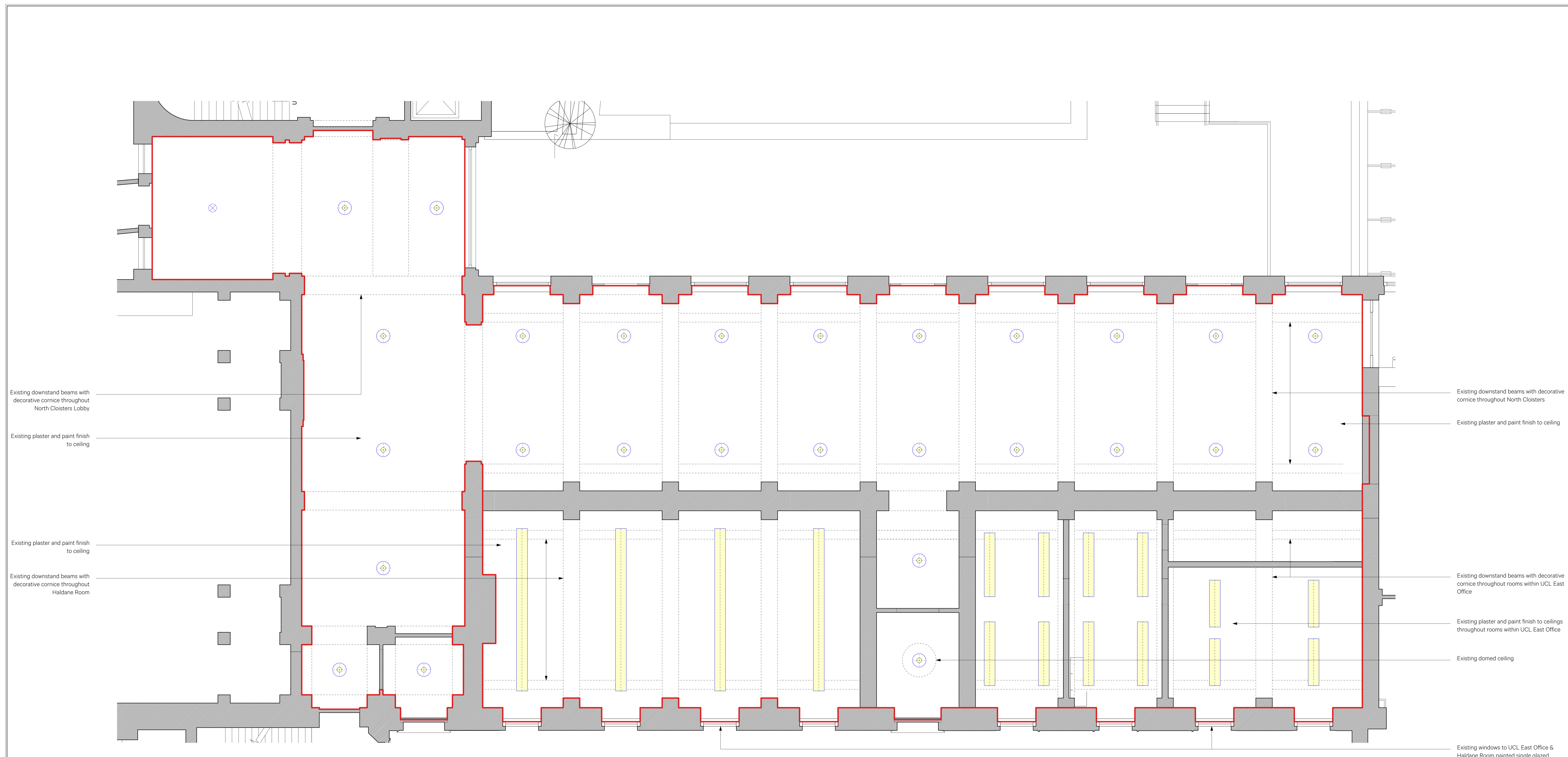
1 North Cloisters Existing RCP 150@A0
