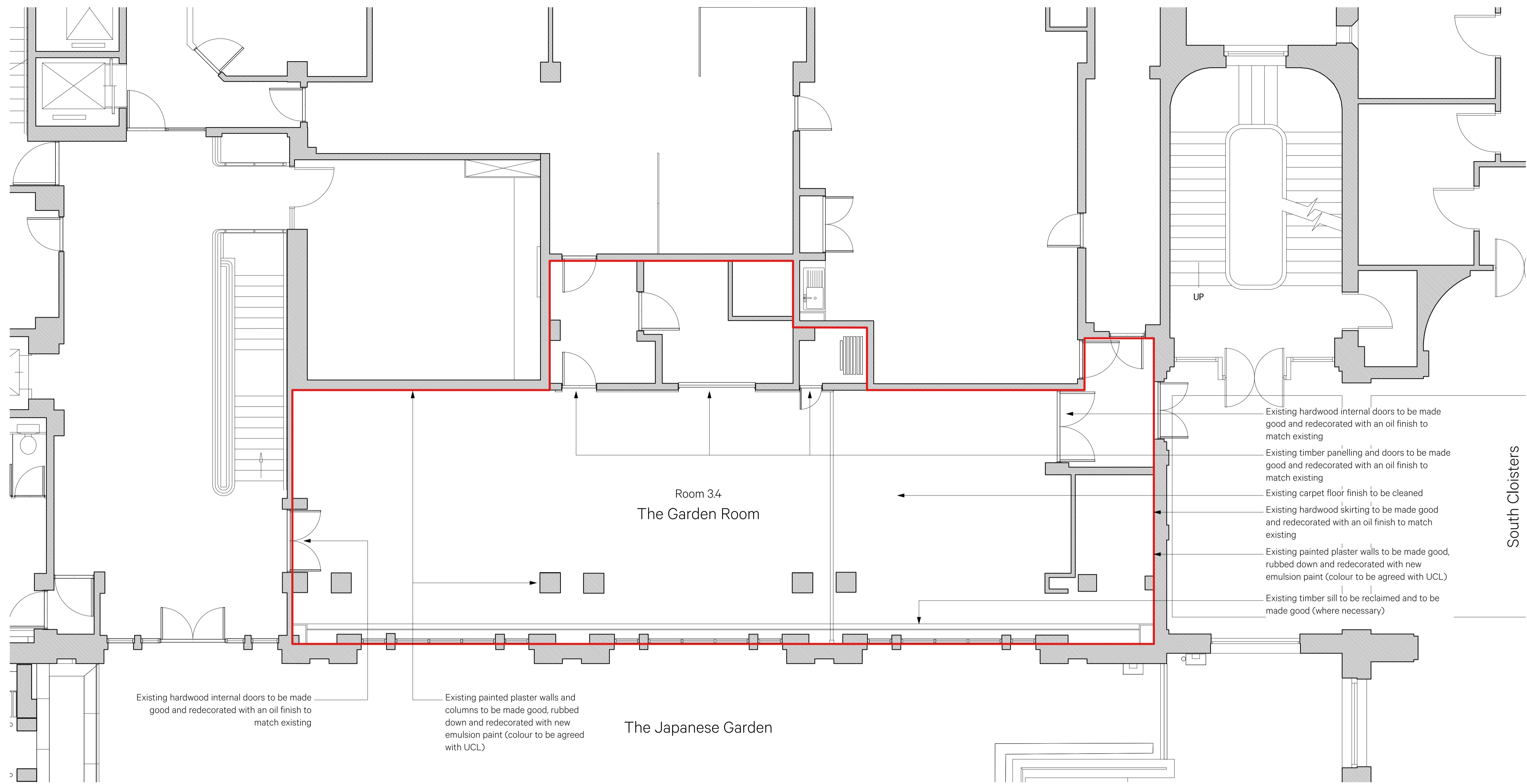
1 Garden Room Floor Plan - Proposed 1:50 @ A0
