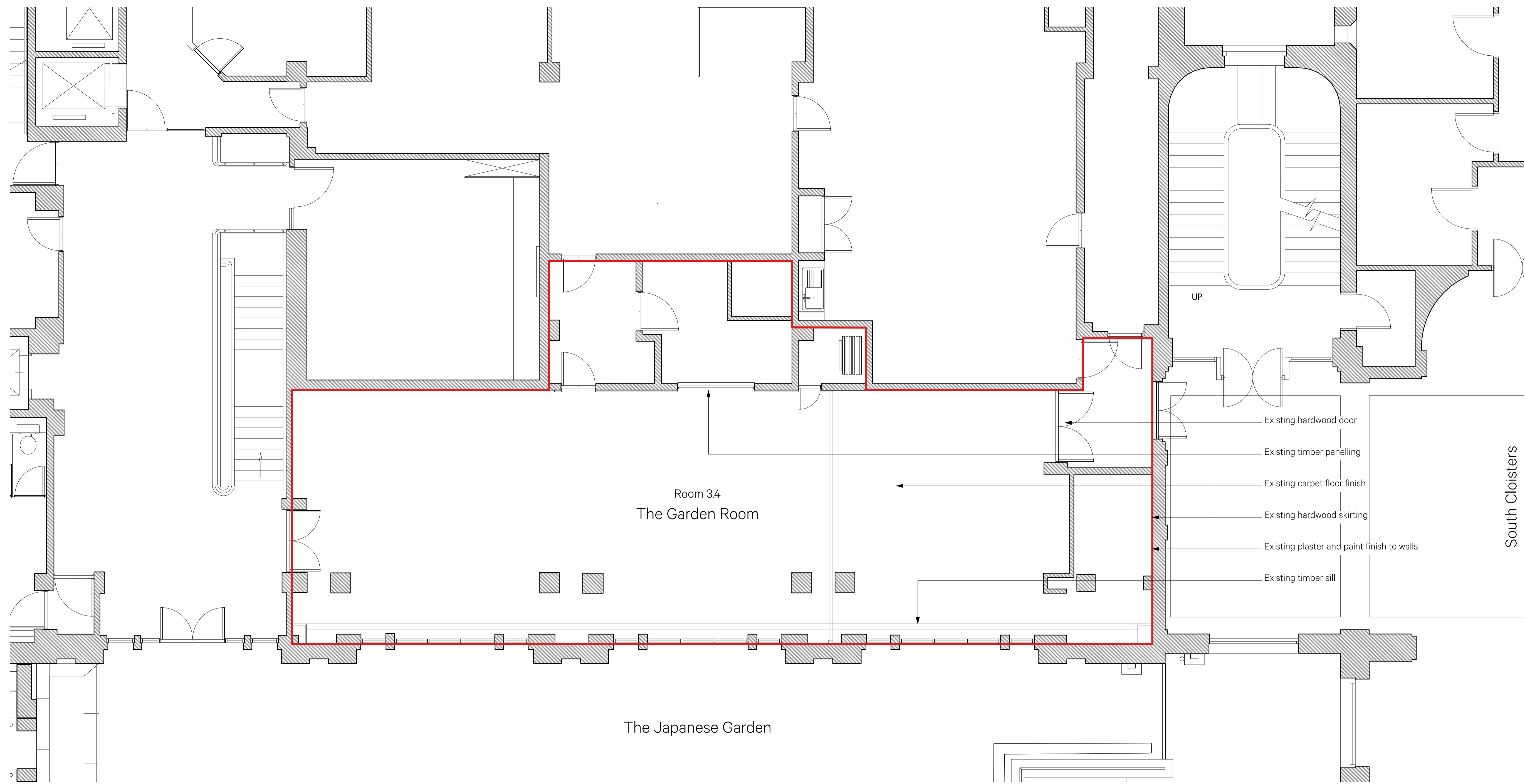
1 Garden Room Floor Plan - Existing 1:50 @ A0
