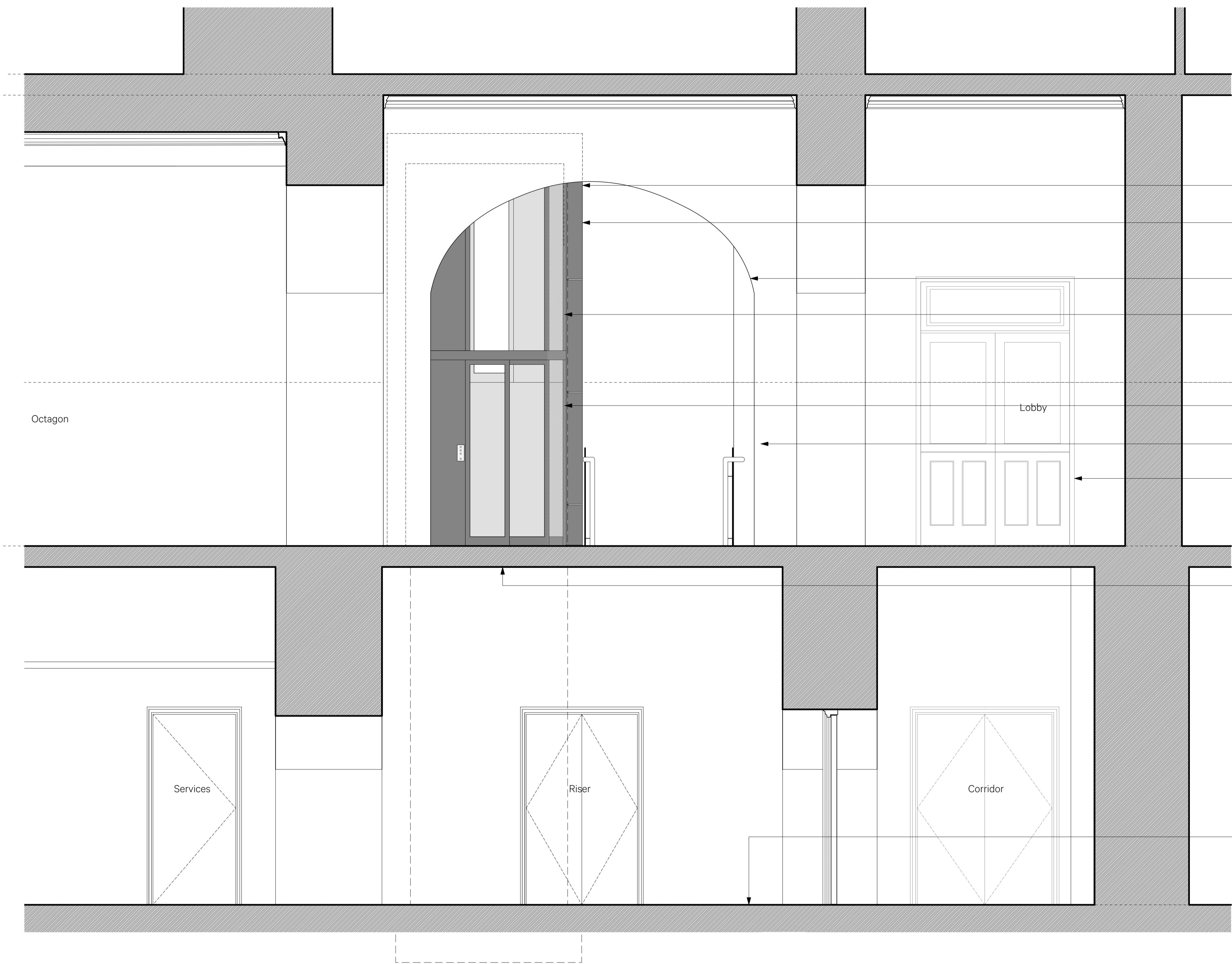
1 New Lift & Stair - Proposed Section G-G 1:25 @ A1
