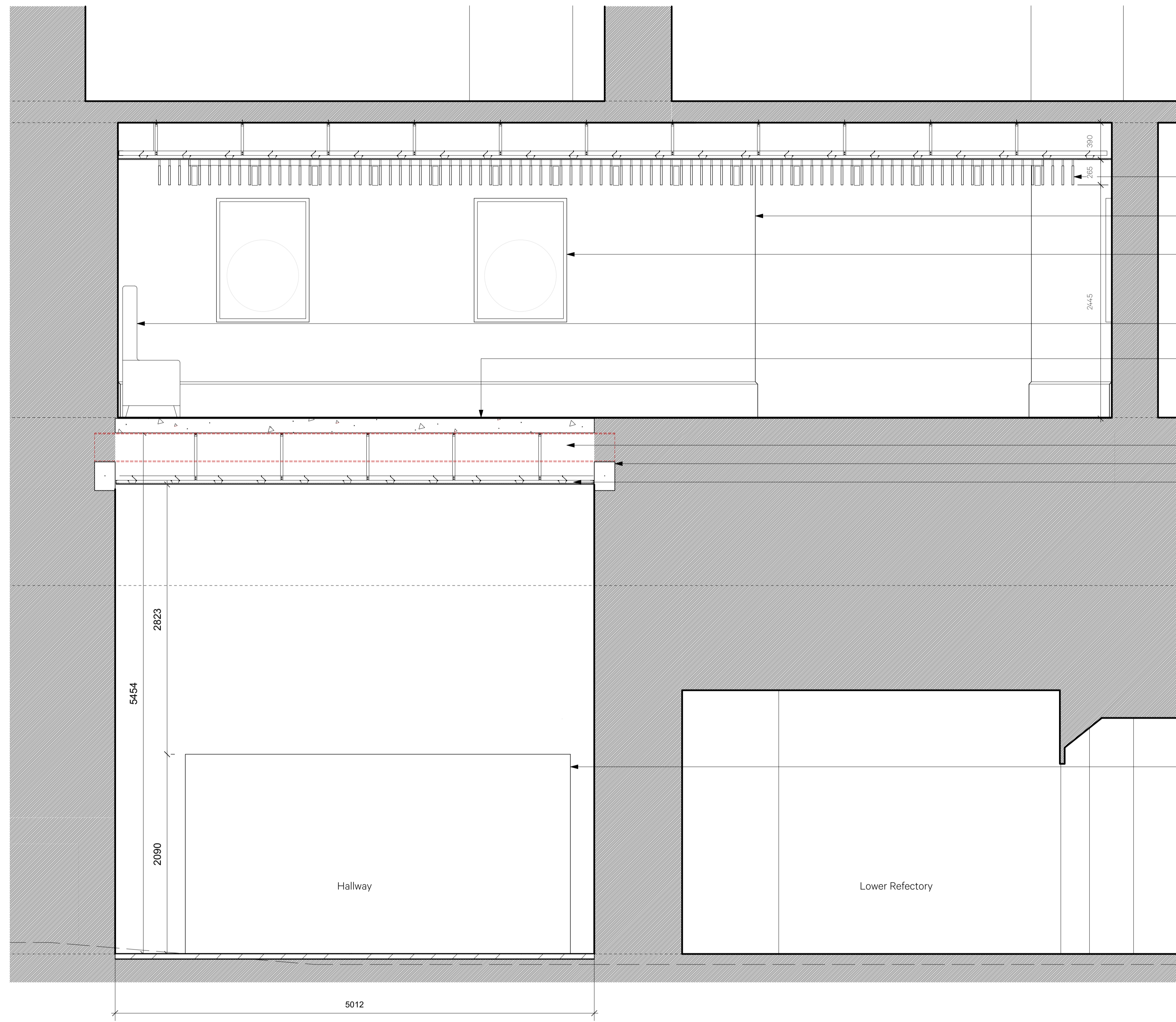
1 New Lift & Stair - Proposed Section B-B 1:25 @ A1
