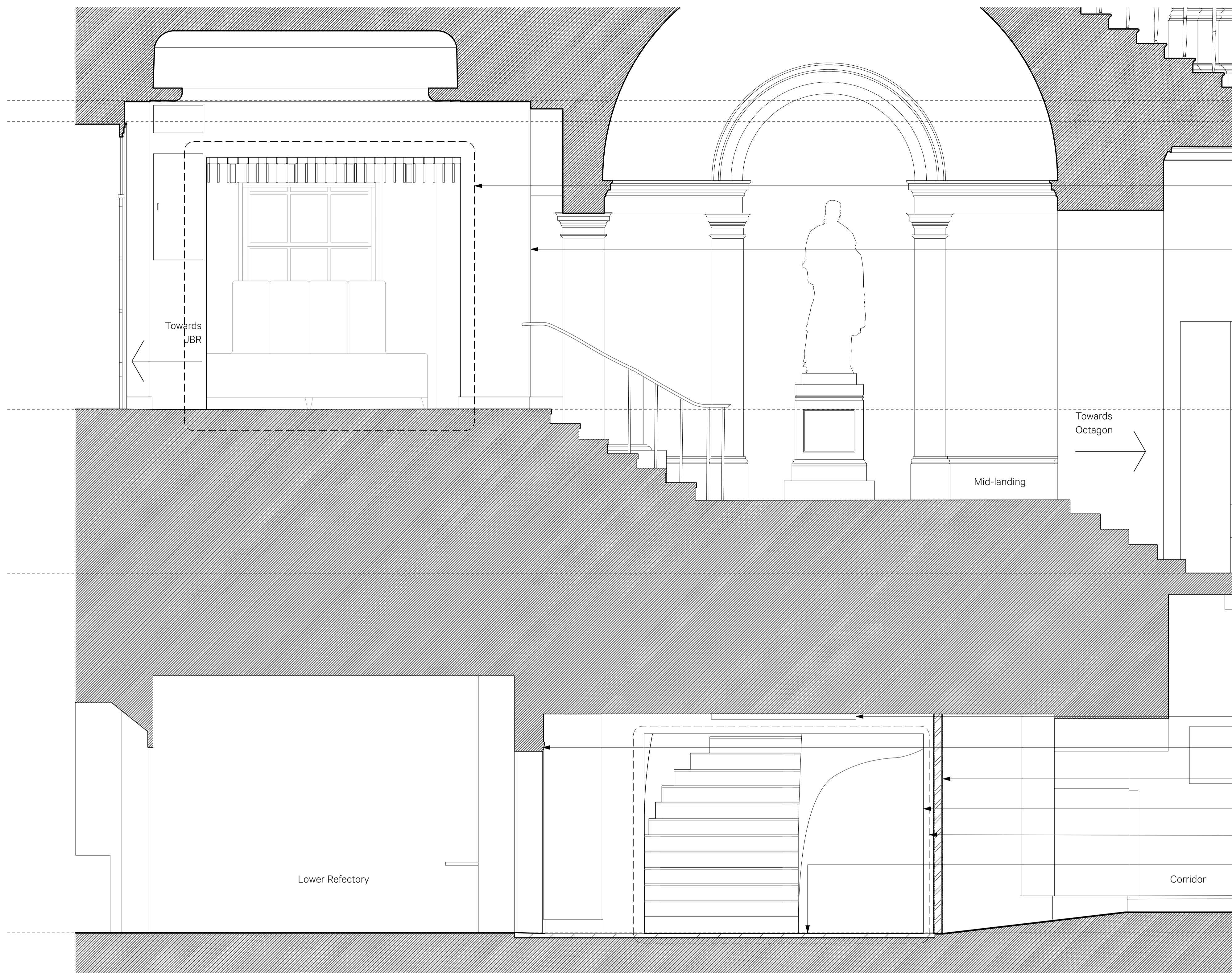
1 New Lift & Stair - Proposed Section A-A 1:25 @ A1
