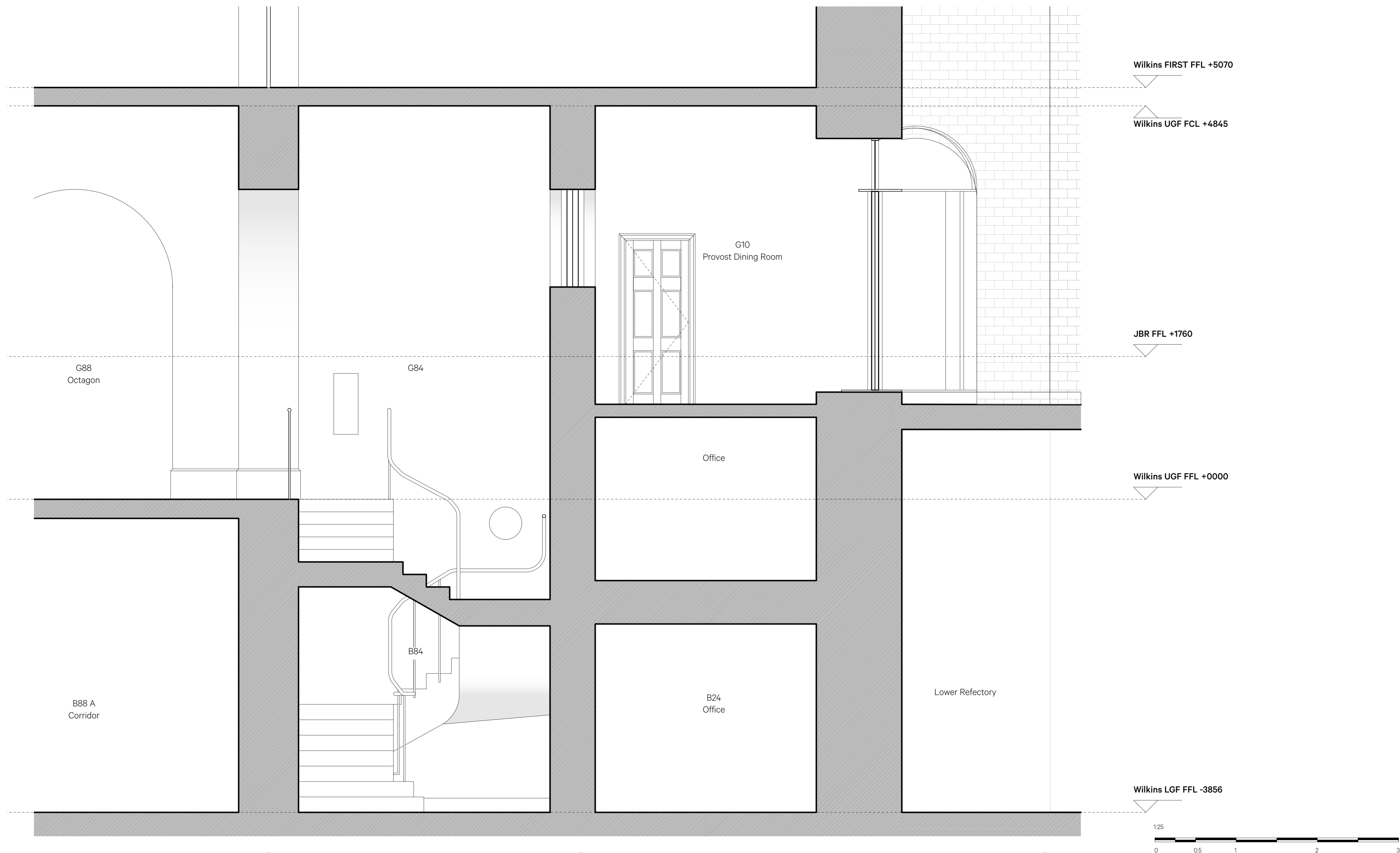
1 New Lift & Stair - Existing Section D-D 1:25 @ A1
