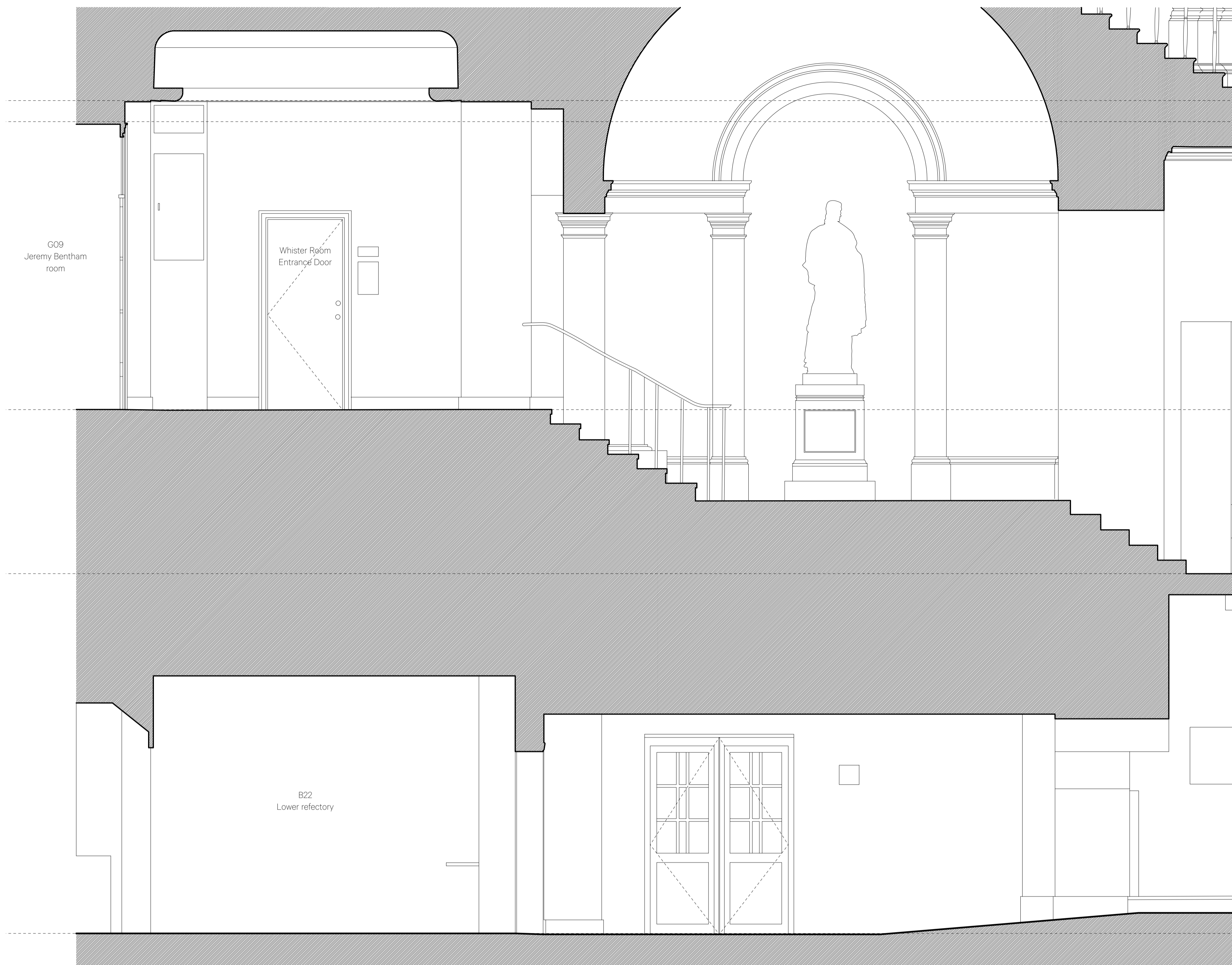
1 New Lift & Stair - Existing Section A-A 1:25 @ A1
