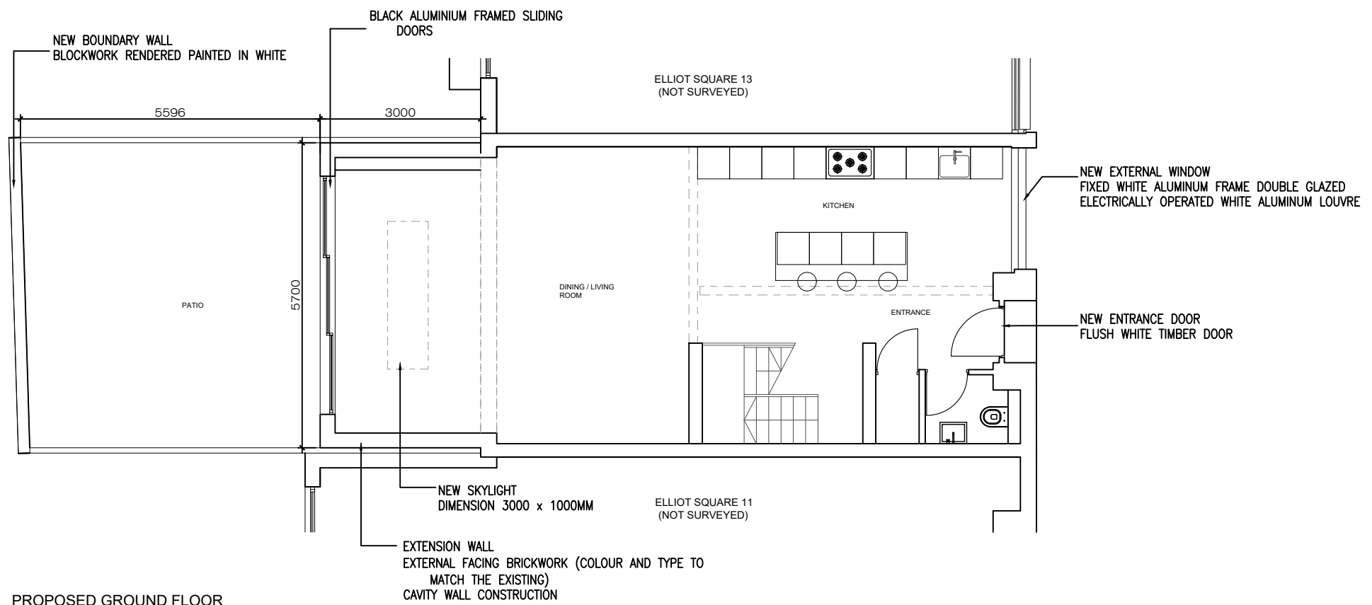
PROPOSED GROUND FLOOR
