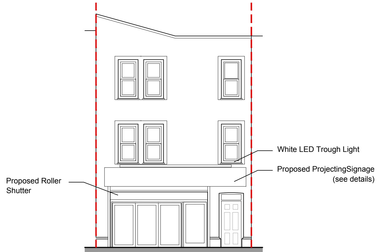
PROPOSED ELEVATION A Pharmacy | Fleet Road
