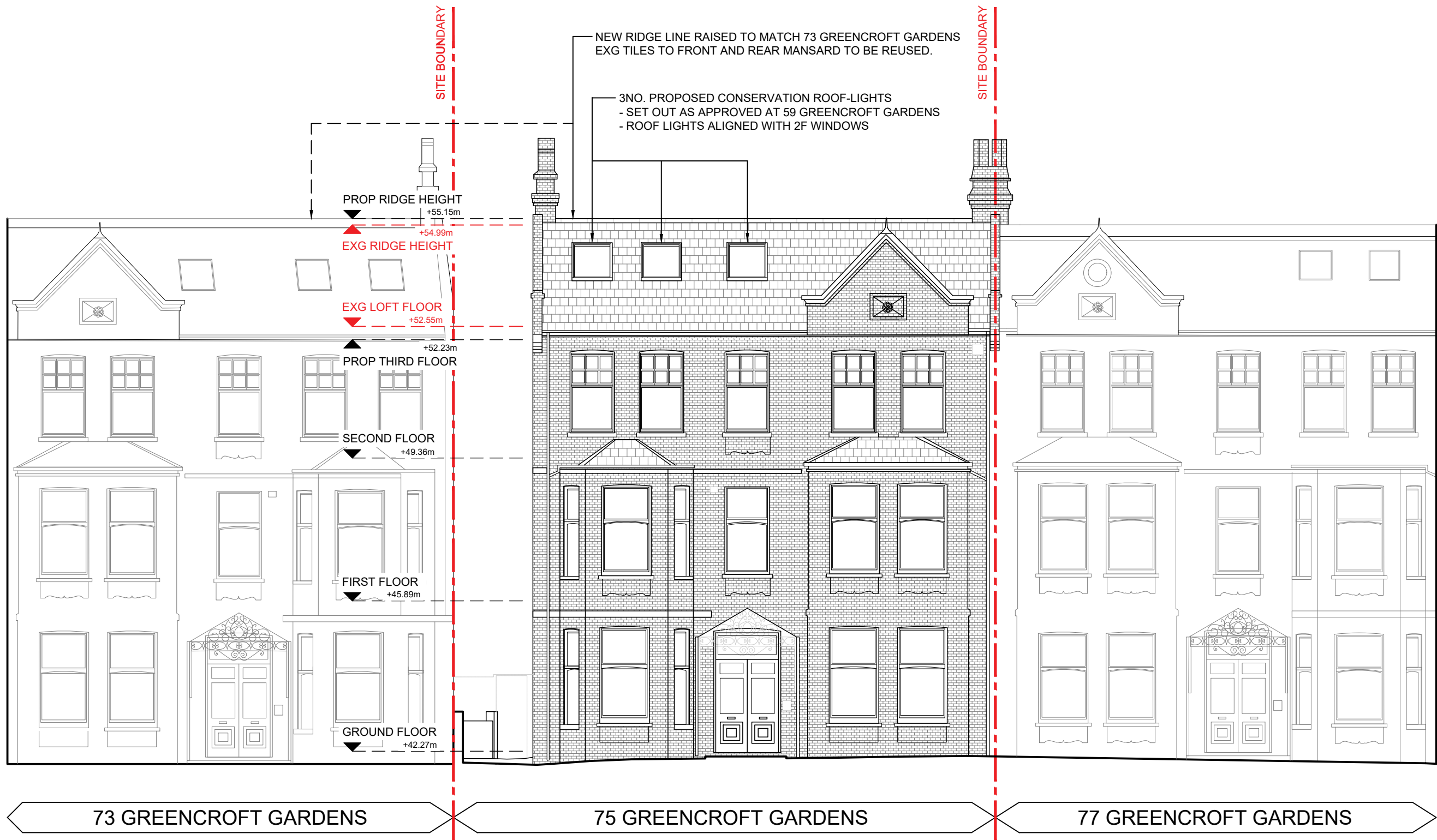
01 PROPOSED - FRONT ELEVATION SCALE // 1:100
