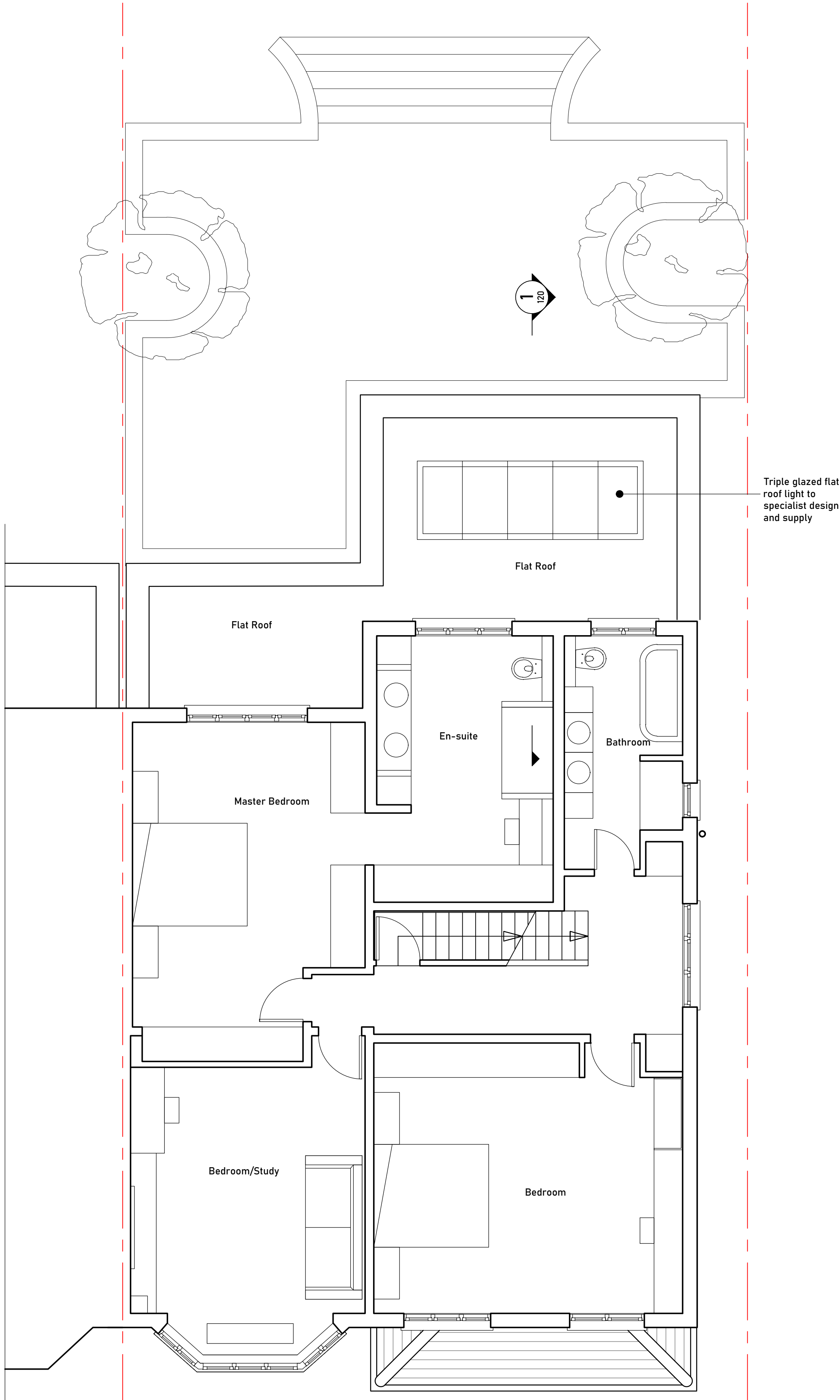
FIRST FLOOR - PROPOSED scale 1:50
