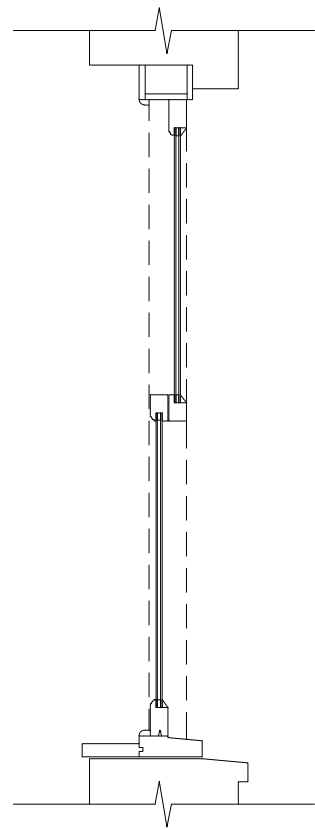
Sash Windows
