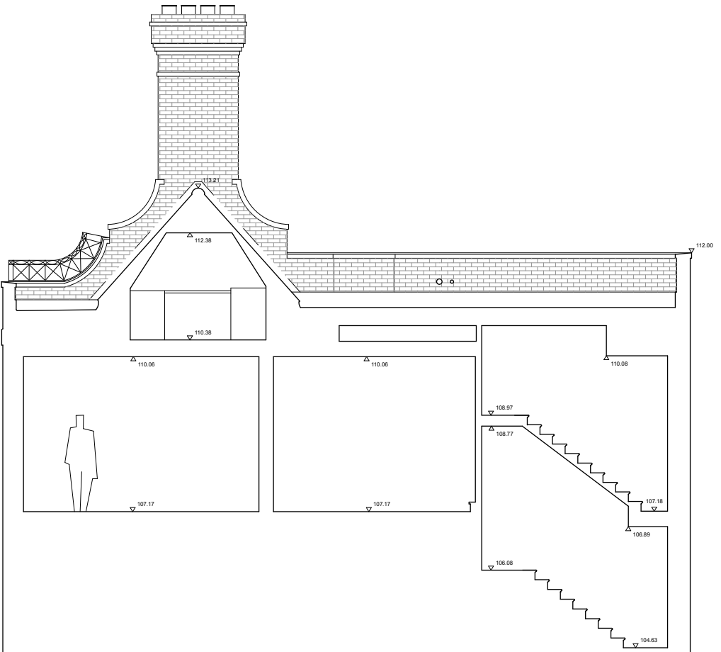
EXISTING SECTION D-D
