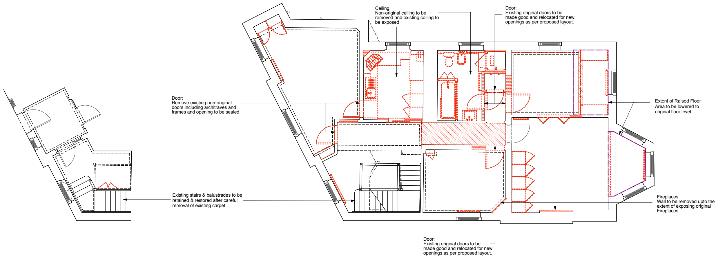
GROUND FLOOR PLAN - DEMOLITION
