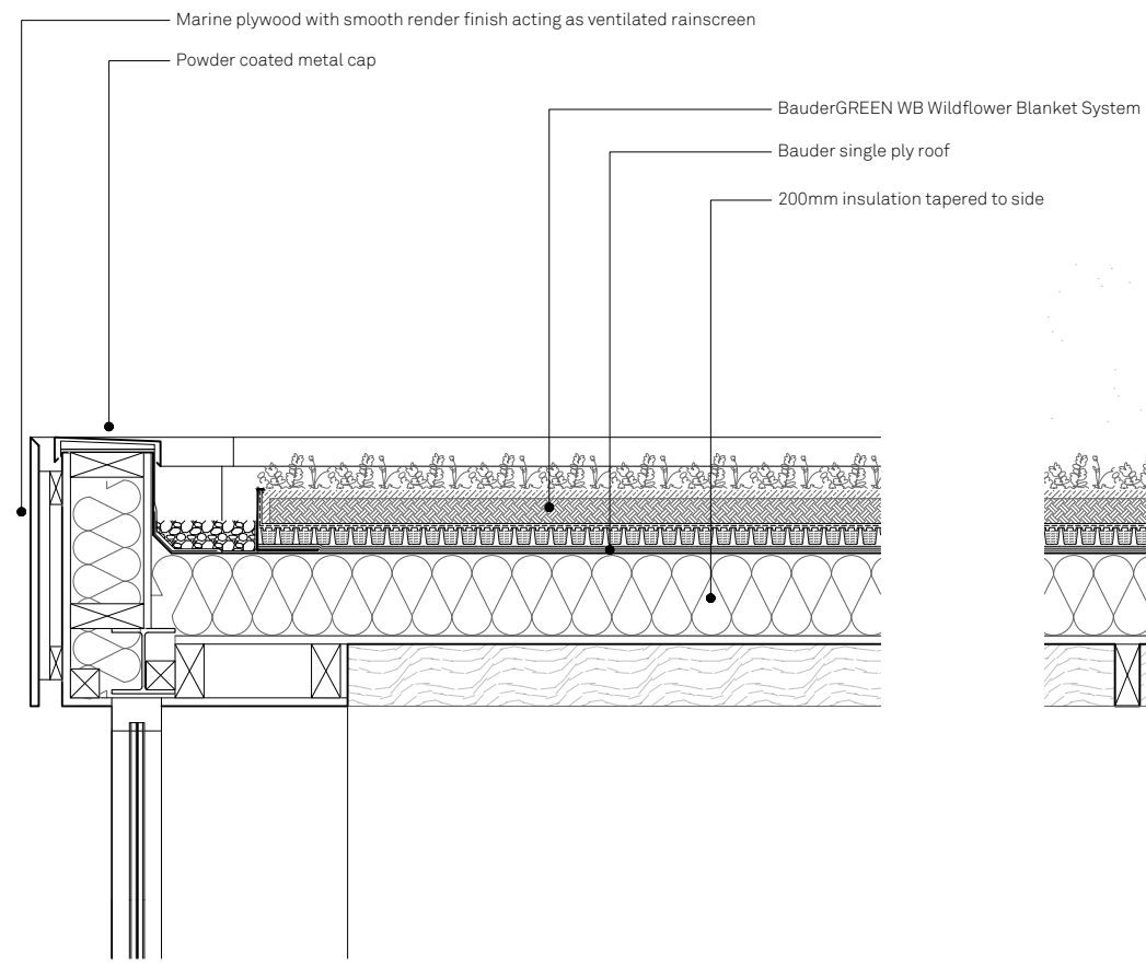
Detail 01 Proposed extension roof 1:20
