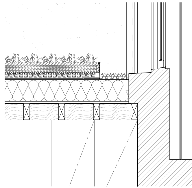
Detail 02 Proposed extension roof 1:20
