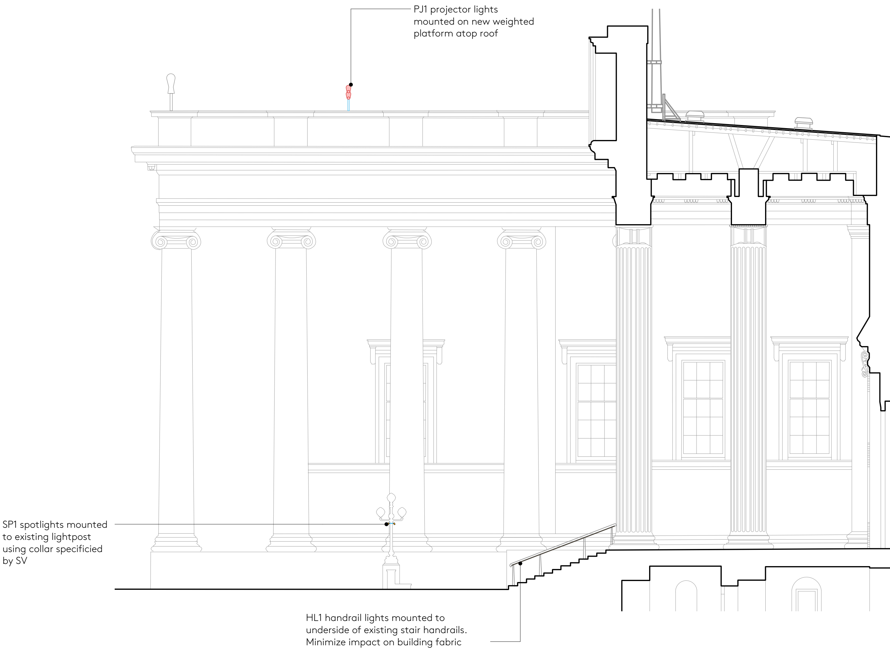
1 South Colonnade - Section (Proposed) Scale: 1:100
