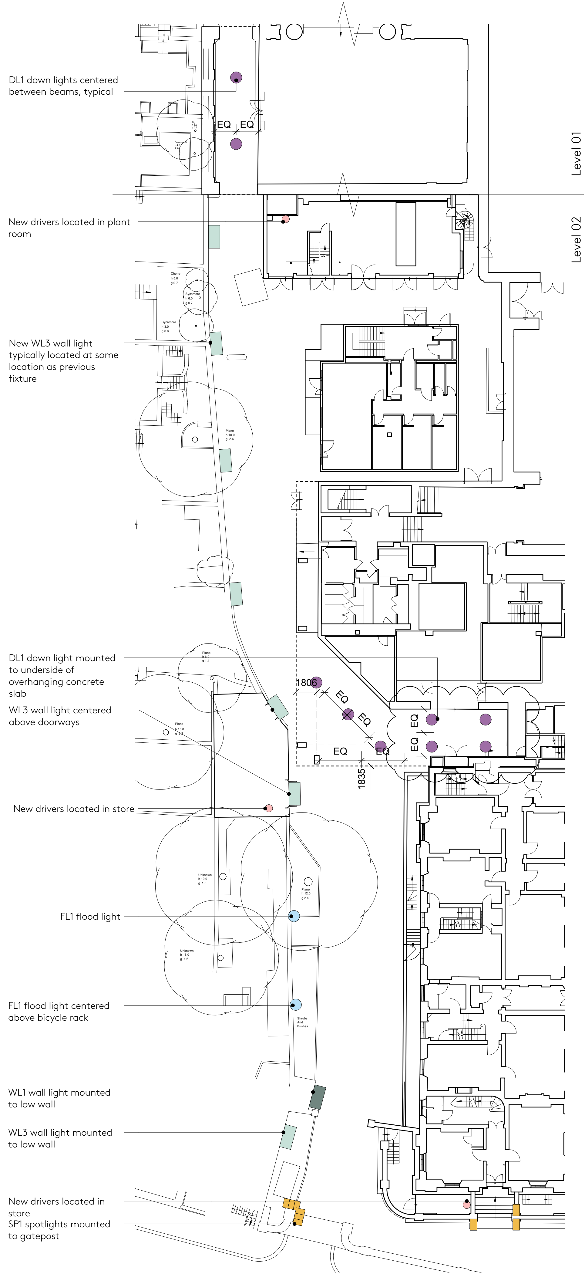
2 West Road - Proposed Plan (South) Scale: 1:200
