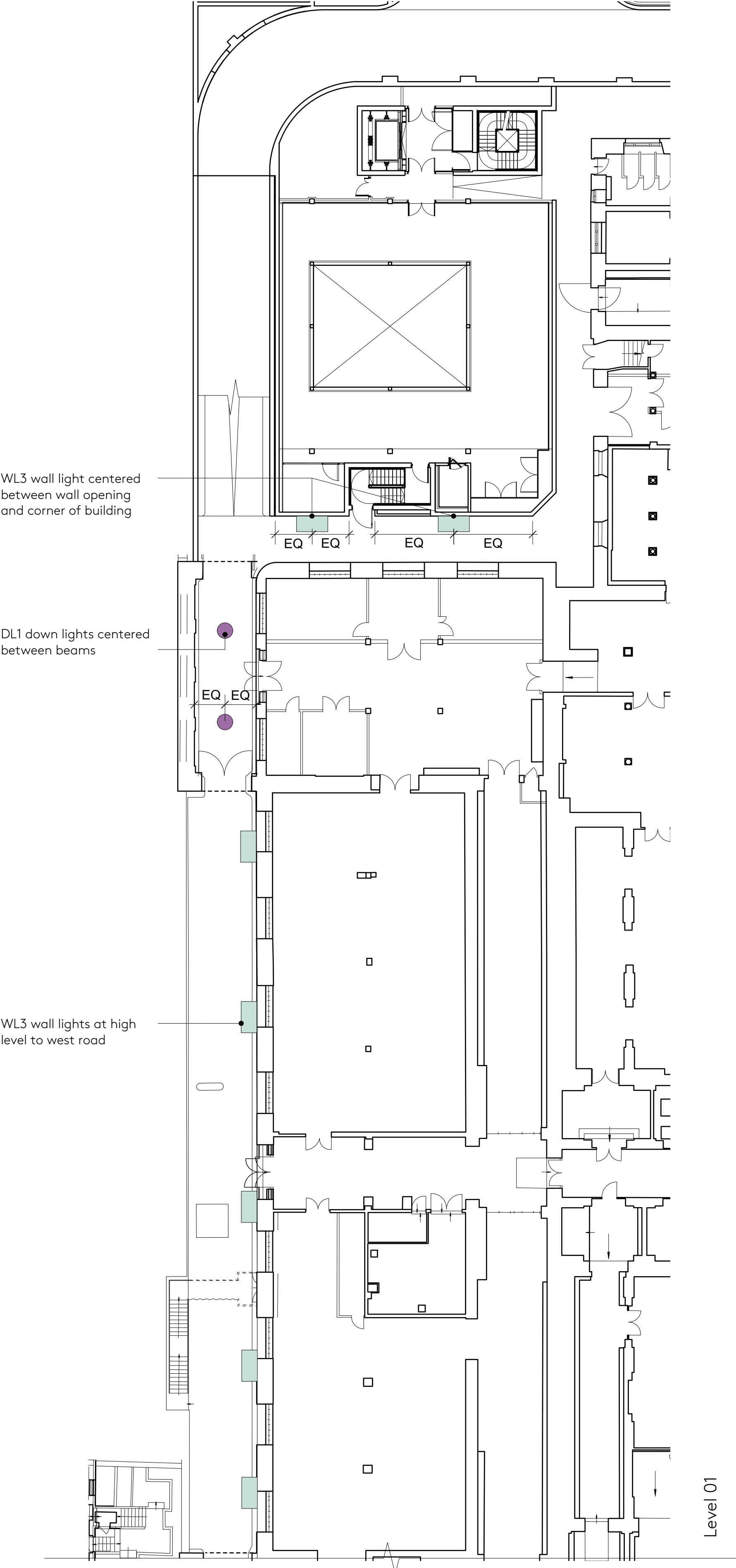
1 West Road - Proposed Plan (North) Scale: 1:200
