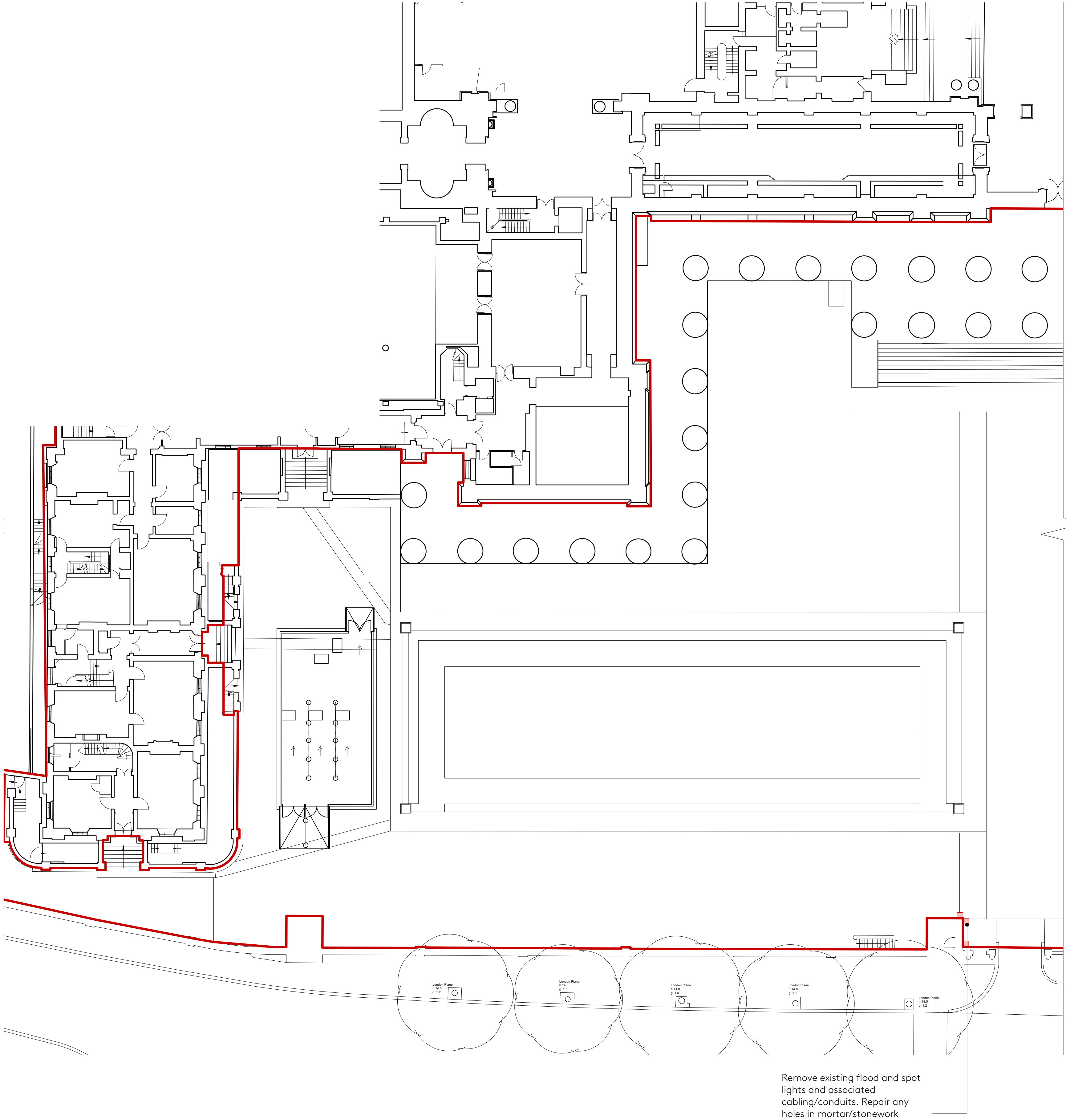
1 Great Russell Street Entrance - Existing Plan (West) Scale: 1:200
