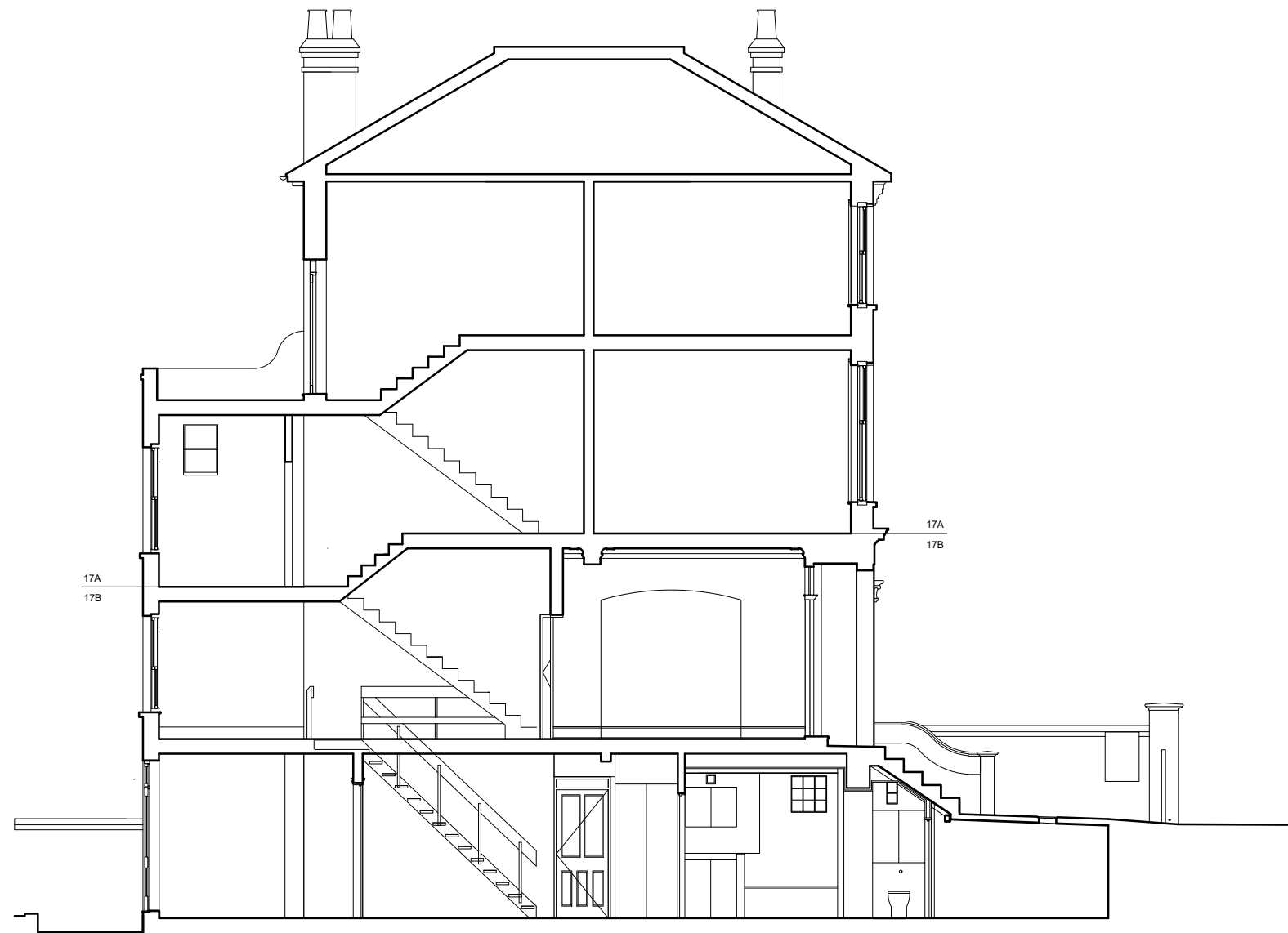
EXISTING SECTION 02
