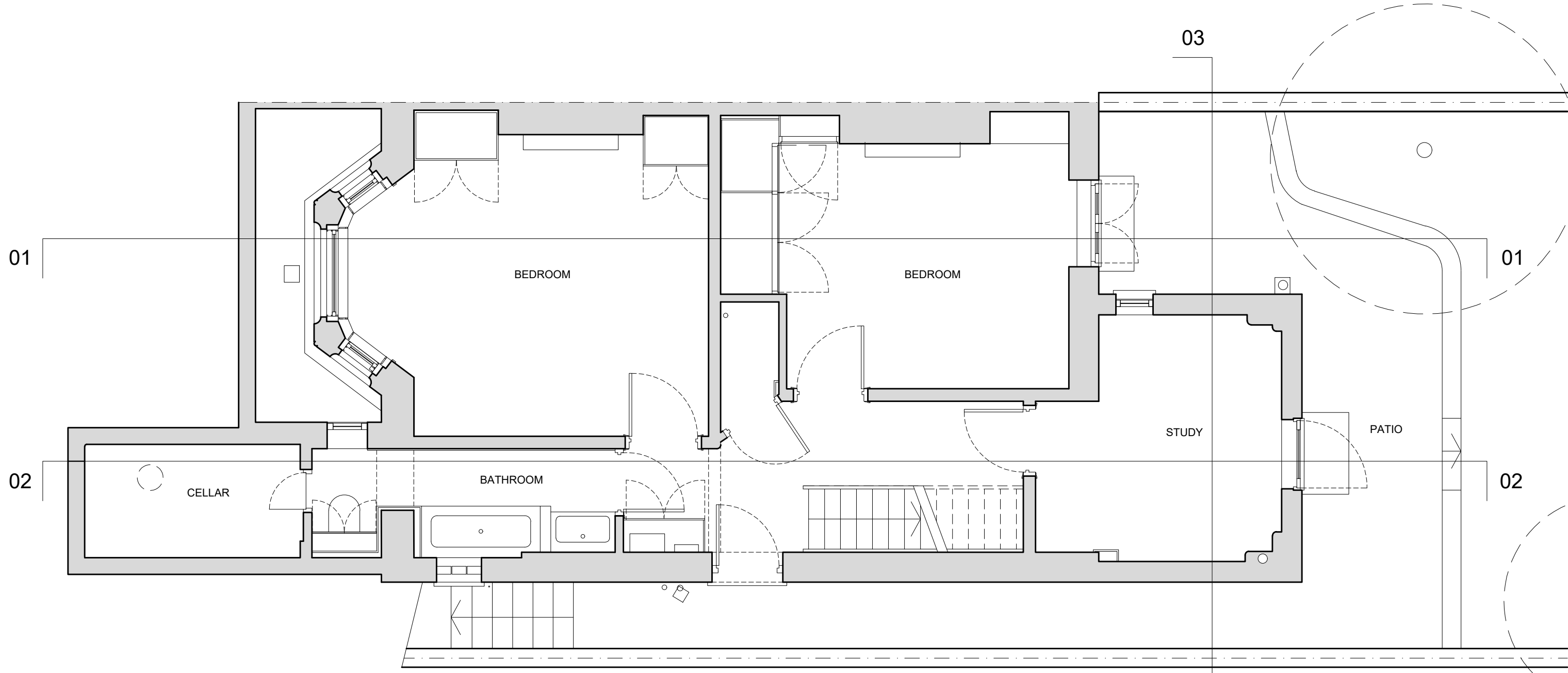
EXISTING LOWER GROUND FLOOR LEVEL PLAN
