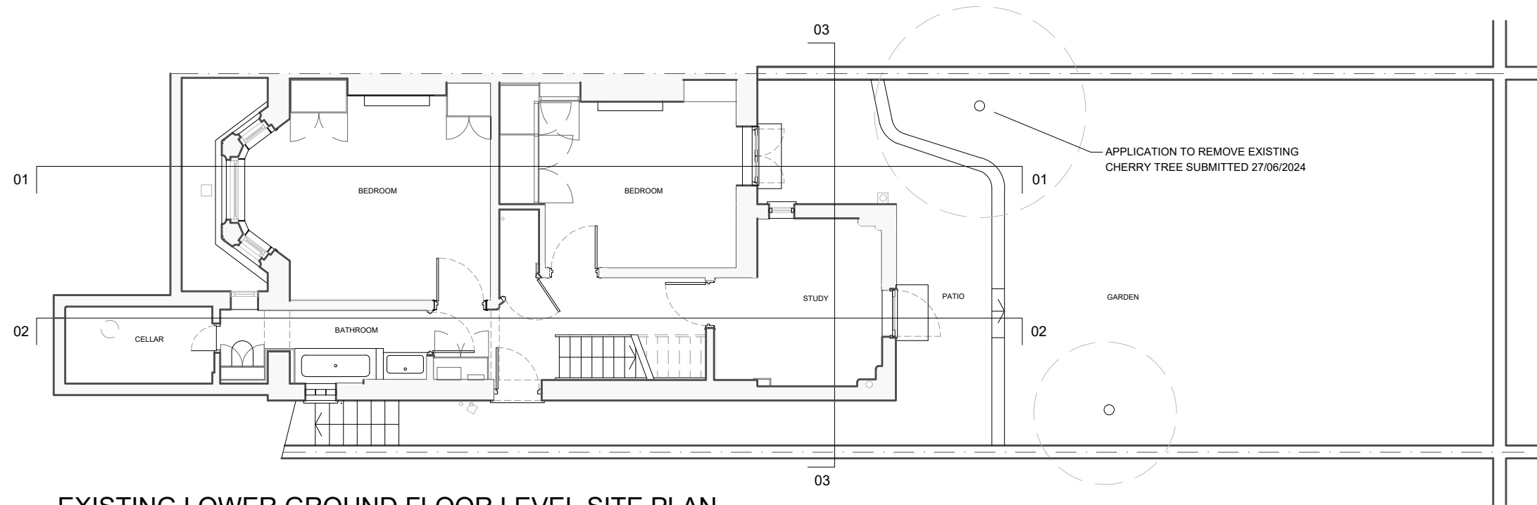
EXISTING LOWER GROUND FLOOR LEVEL SITE PLAN
