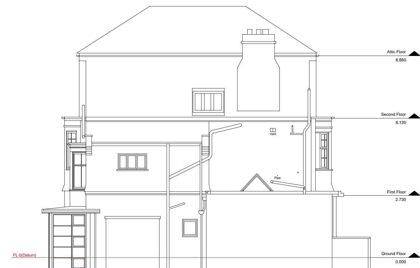
Left Elevation
