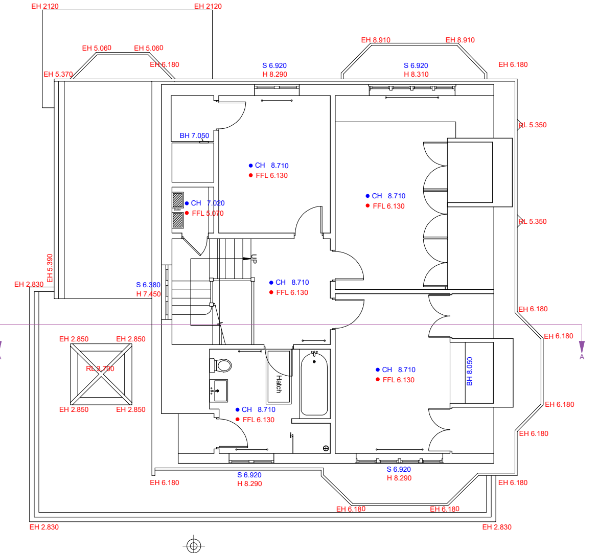
Second Floor
