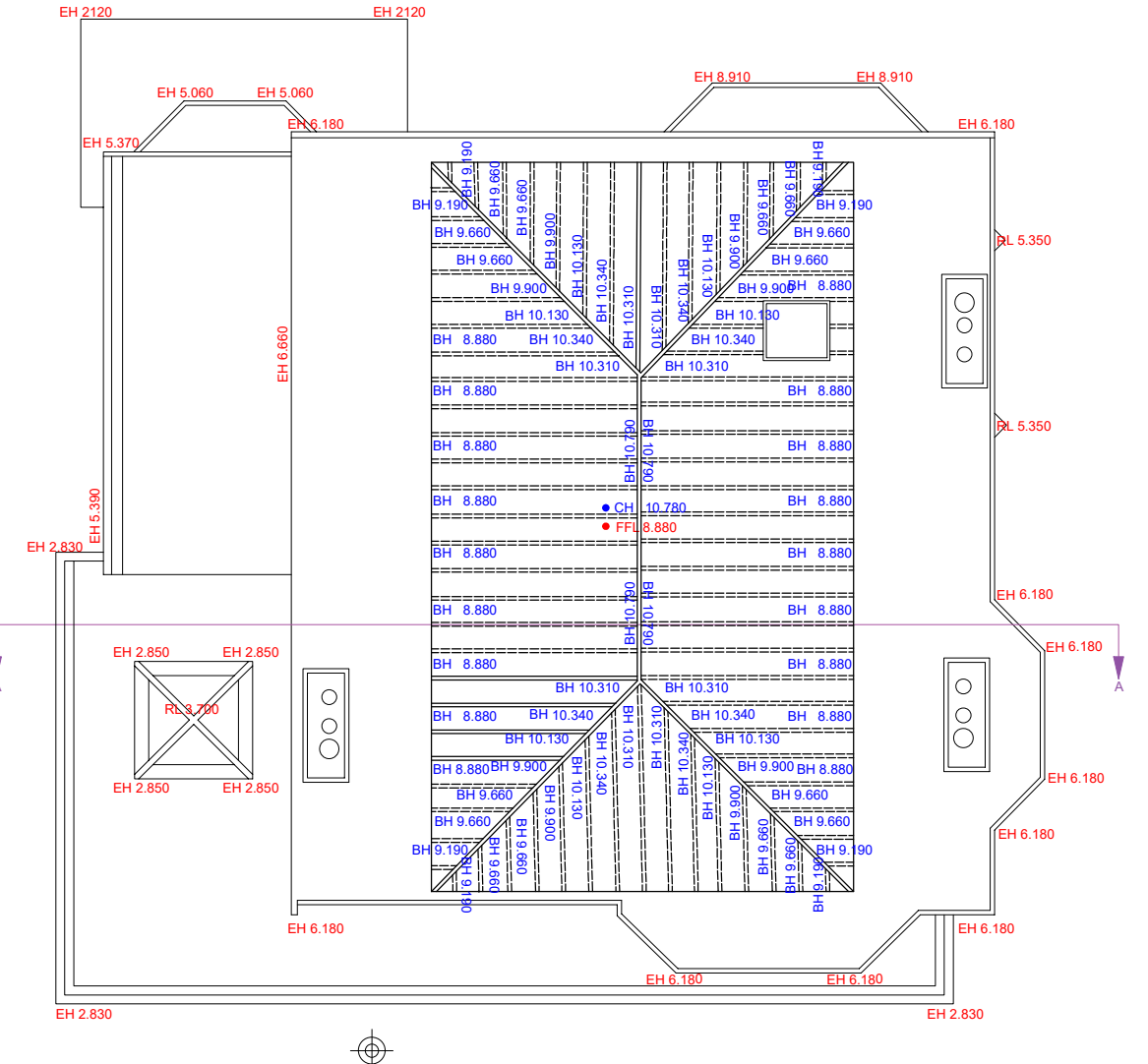
Attic Floor
