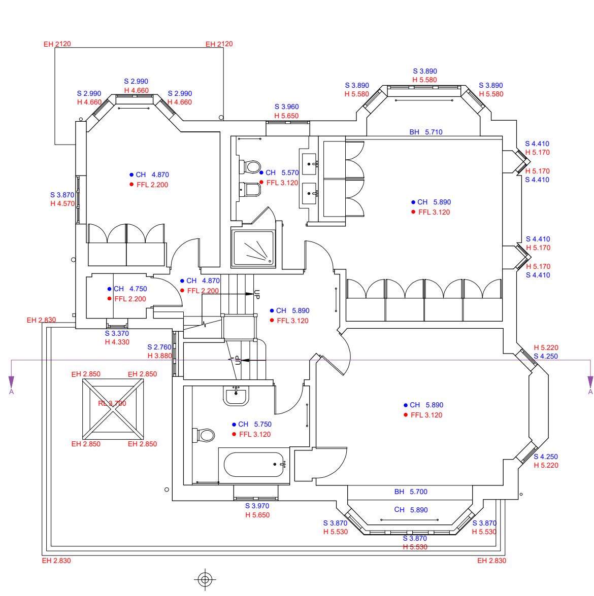
First Floor
