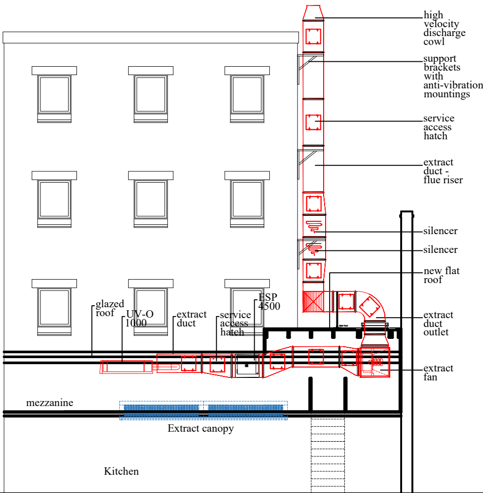
PROPOSED REAR ELEVATION - SECTION C-C
