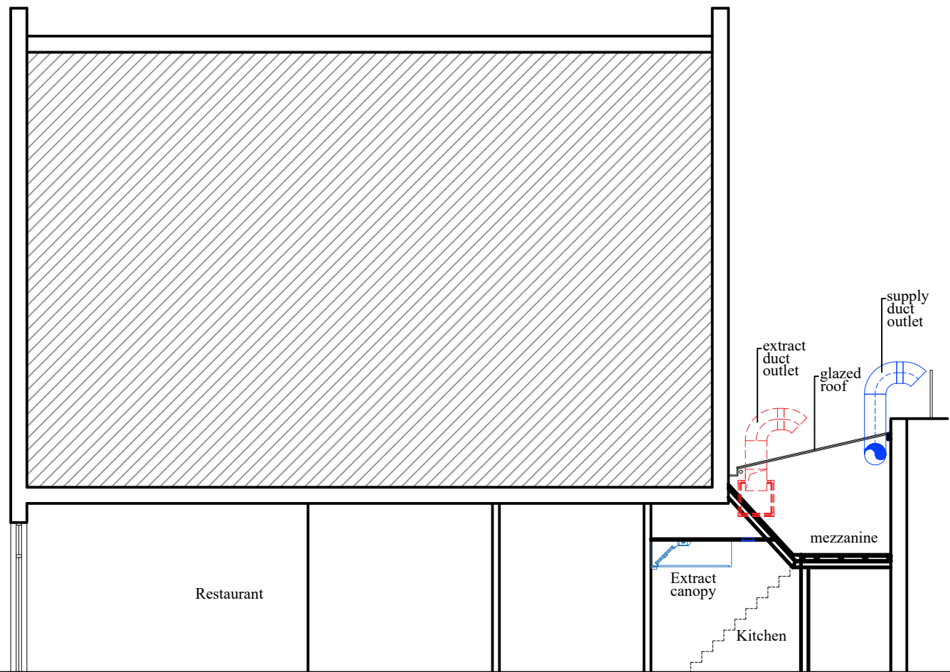
EXISTING SECTION B-B
