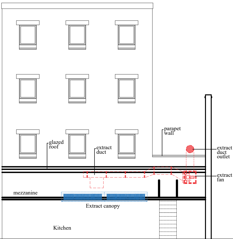
EXISTING REAR ELEVATION - SECTION C-C
