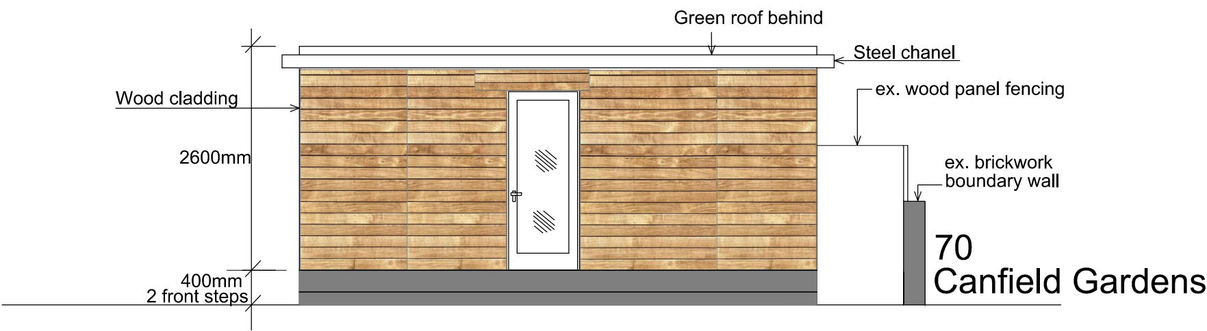
WEST / FRONT ELEVATION
