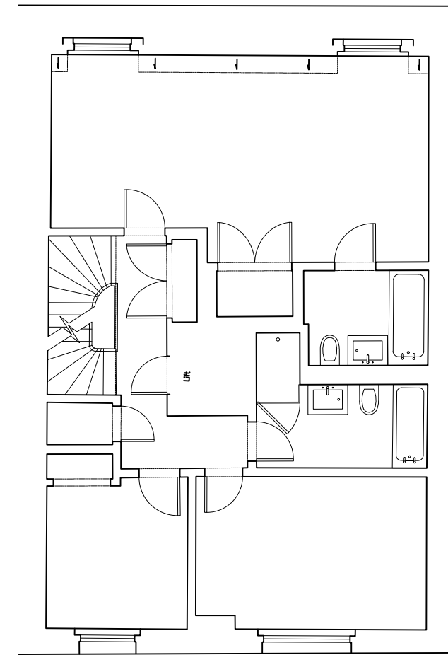
Third Floor Level
