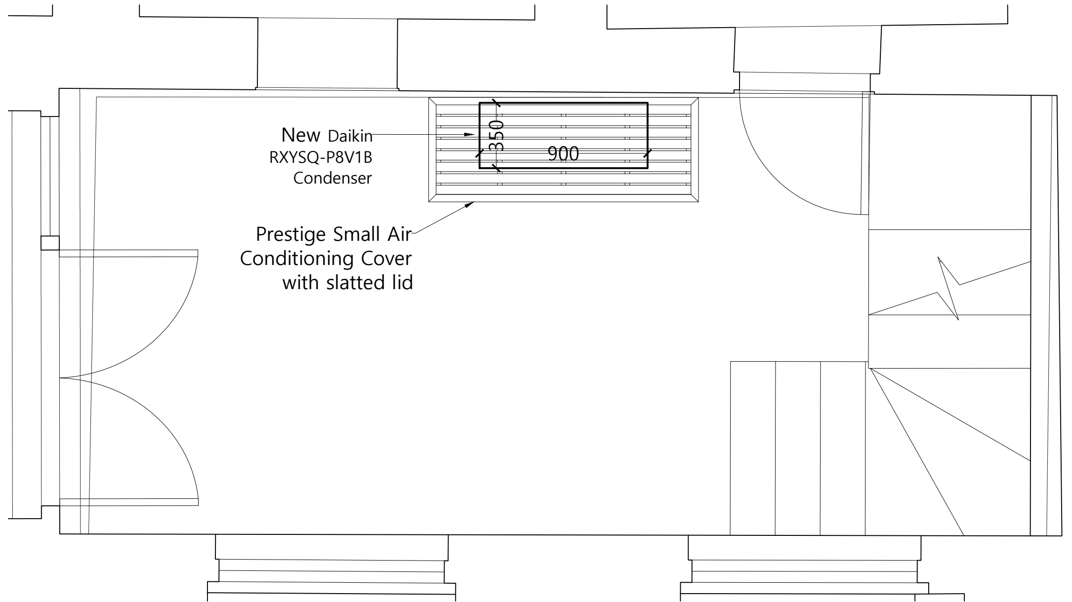
Lower Courtyard Plan 1:20 @ A3
