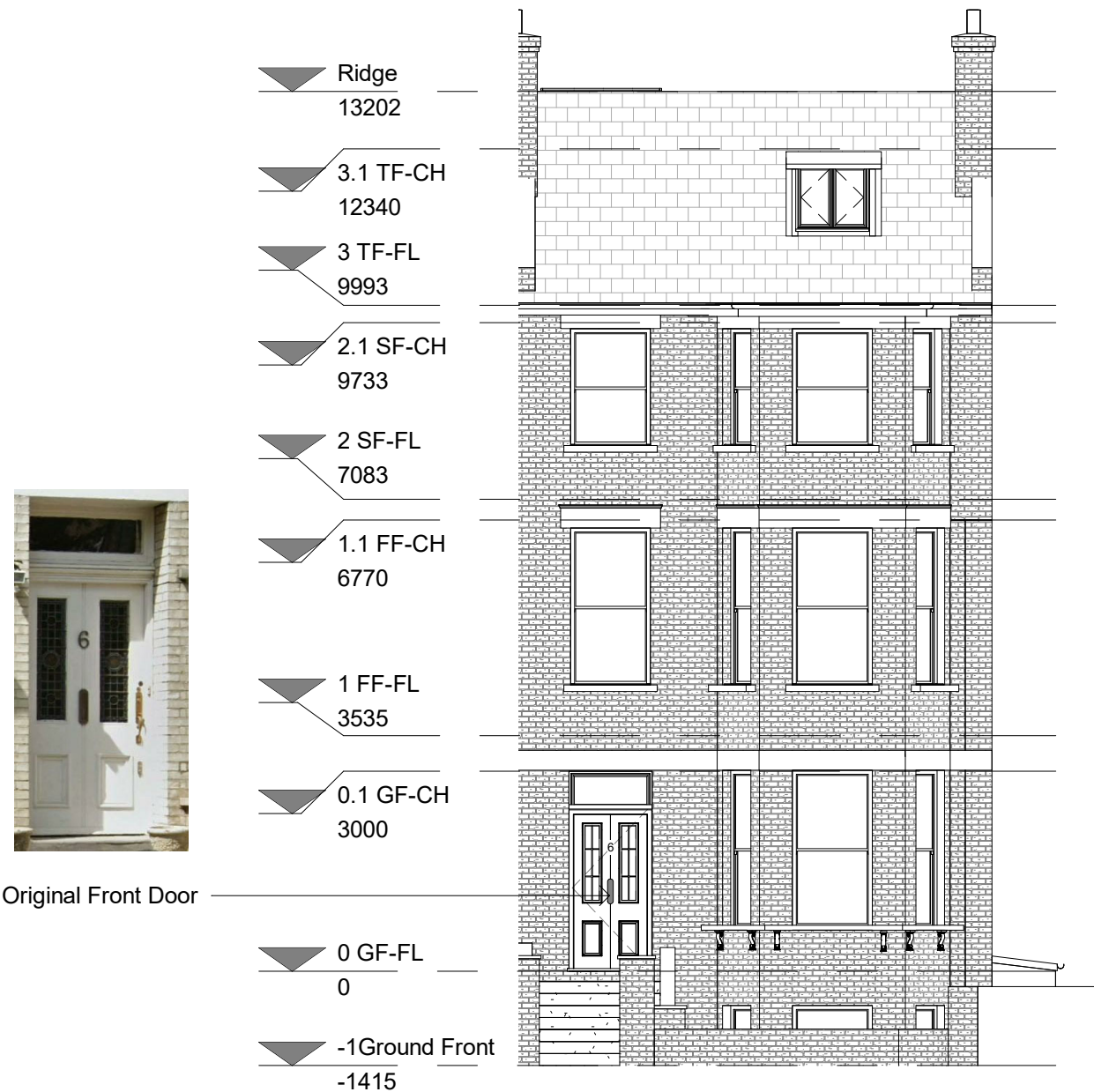
Original Front Elevation 1 : 100
