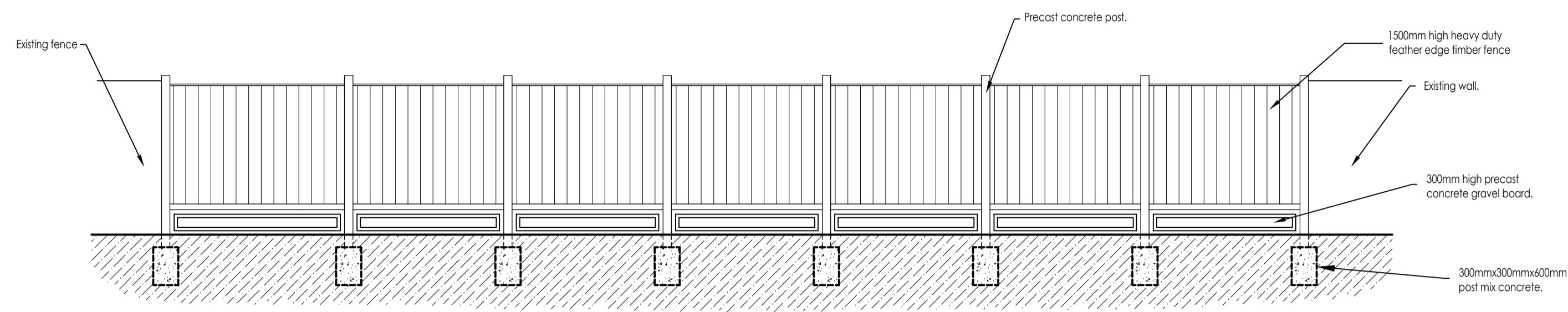
Proposed Elevation Scale 1:50
