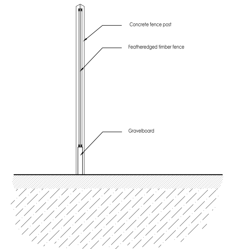
Proposed Fence Typical Section Scale 1:20
