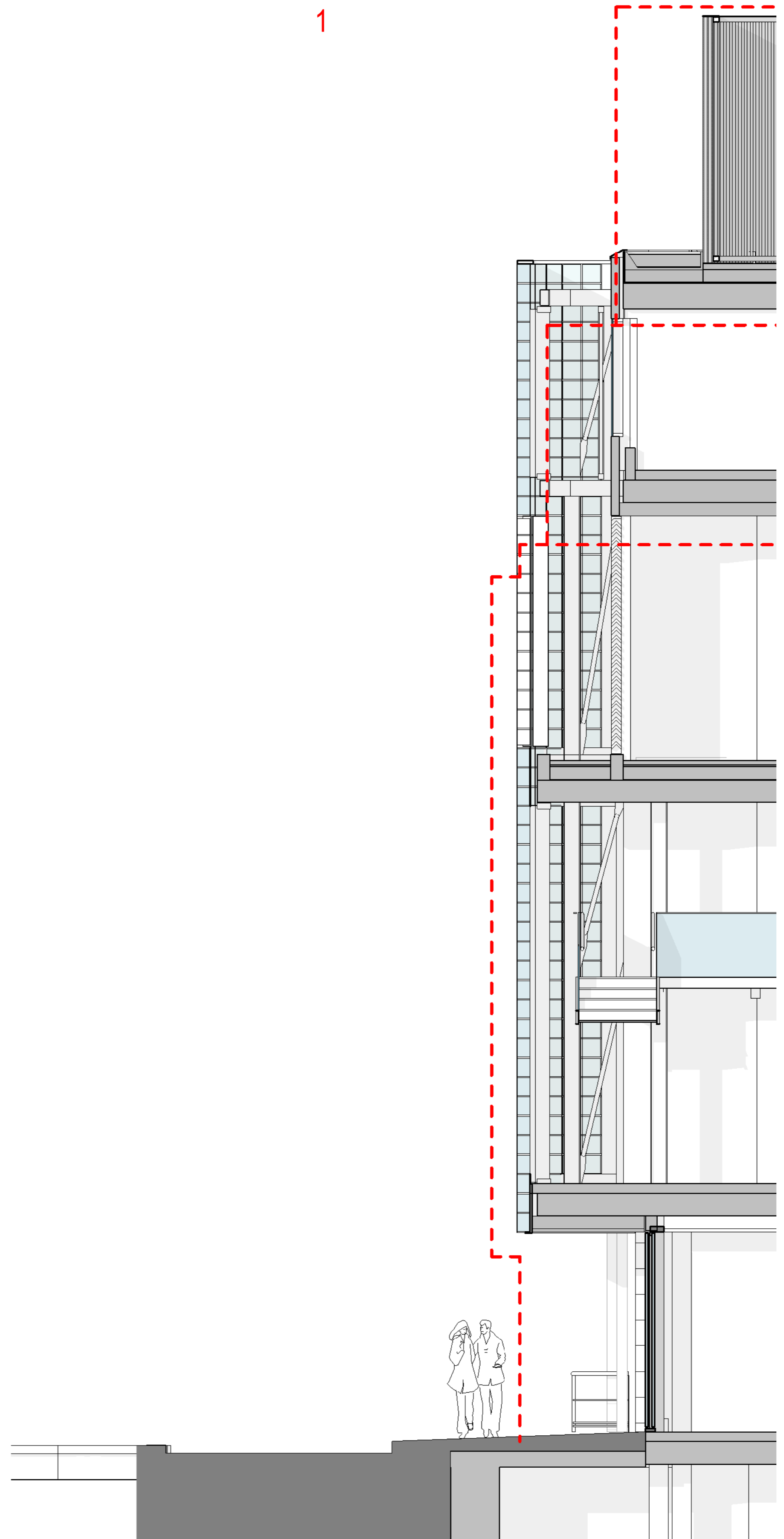
1 FURNIVAL ST 40 SETTING OUT SECTION 1:50
