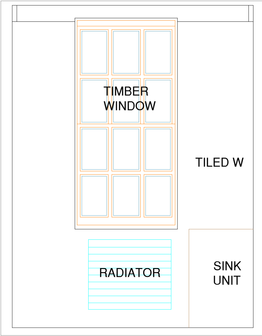
BATHROOM ELEVATION 1:20 Scale
