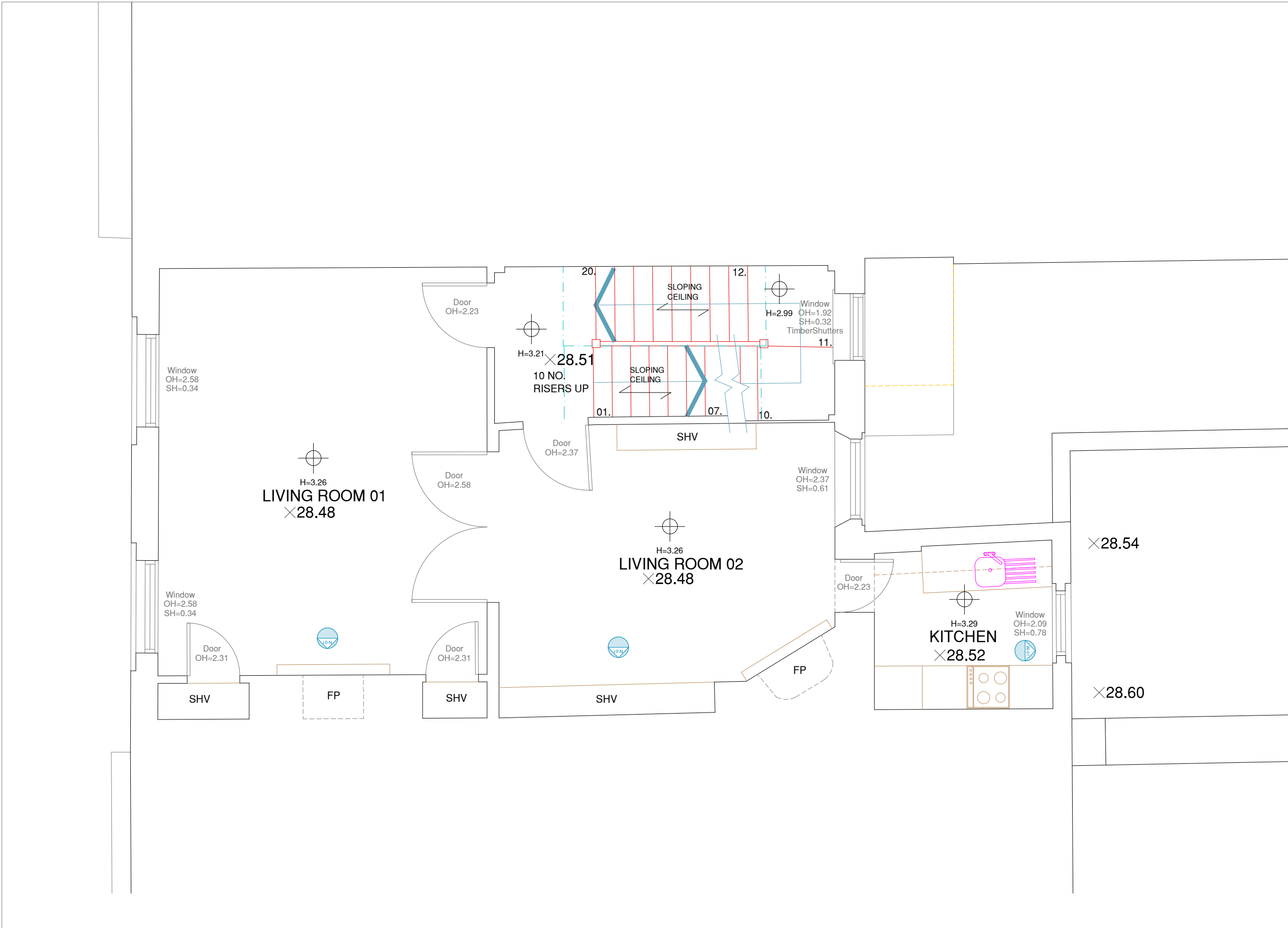
FIRST FLOOR PLAN 01 1:50 Scale
