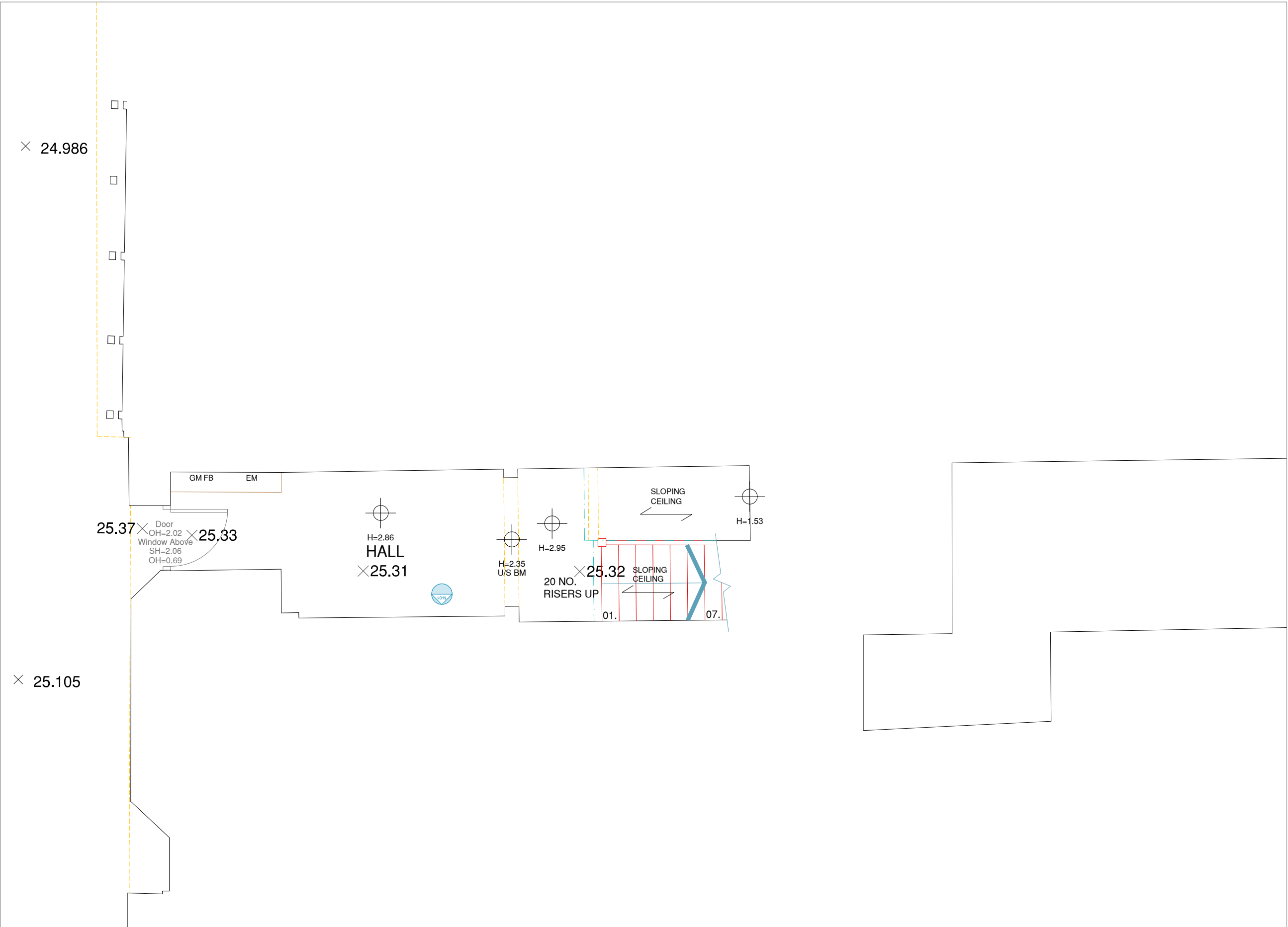
GROUND FLOOR PLAN 01
