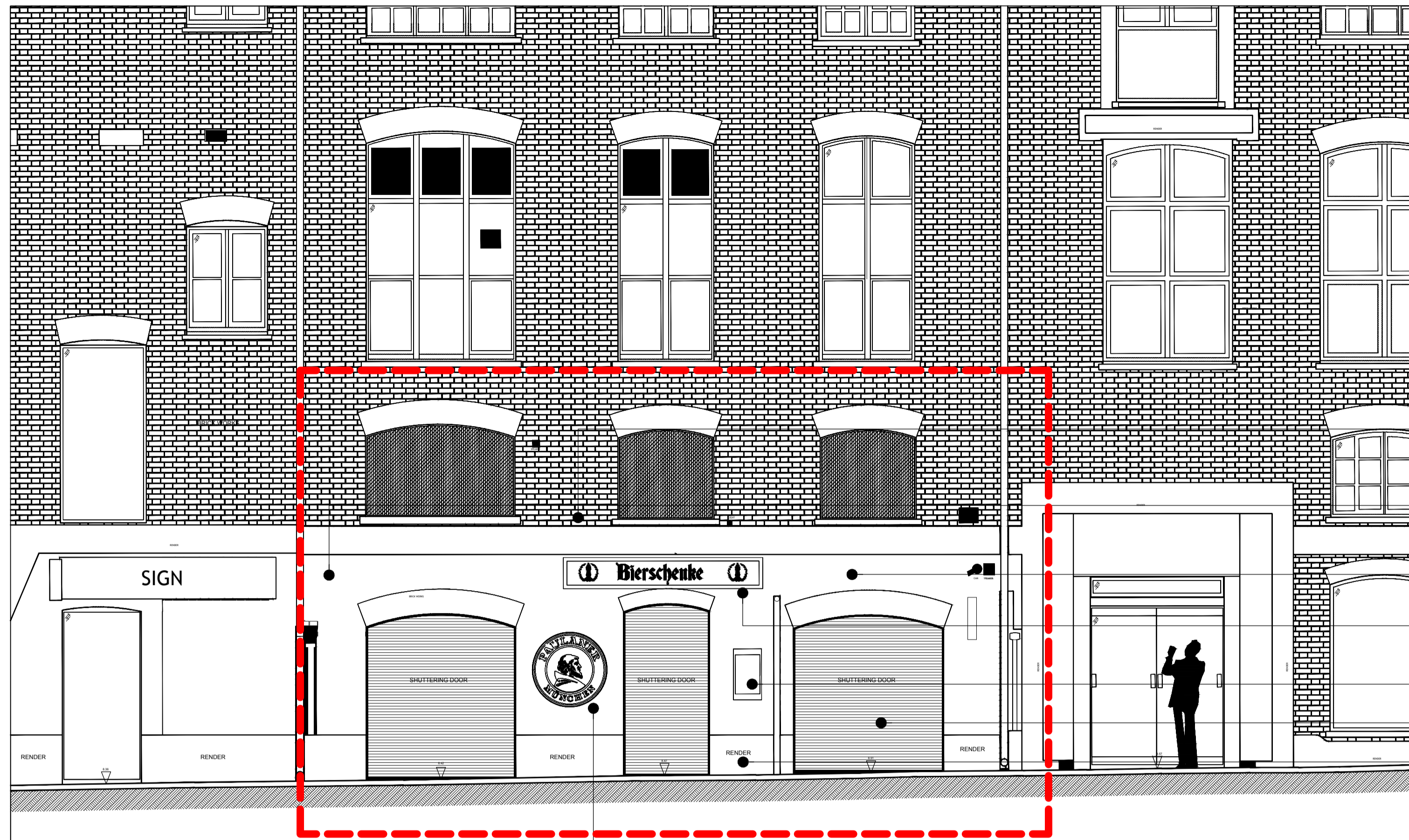
EXISTING EARLHAM STREET FRONT ELEVATION SCALE 1:50
