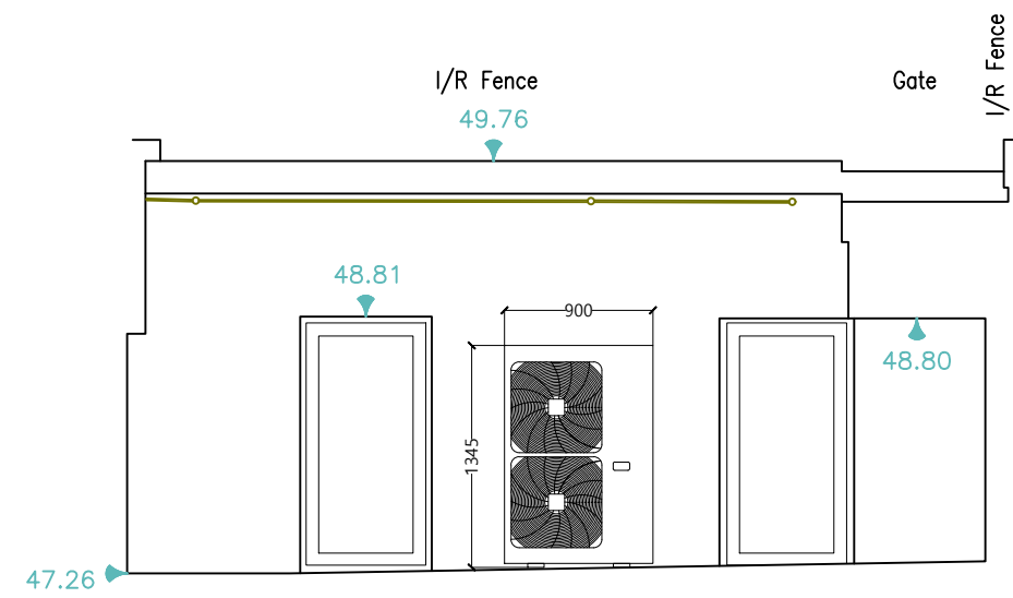
4 - Basement Elevation - Daikin Unit
