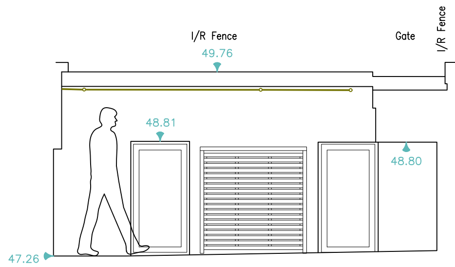
4 - Basement Elevation - Proposed Timber Enclosure
