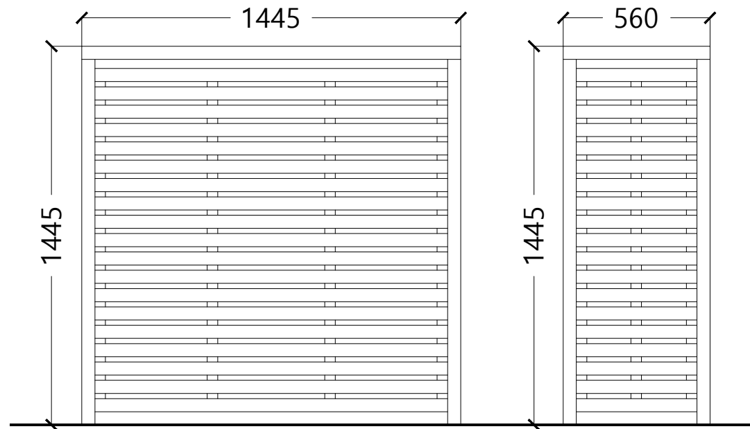
FRONT ELEVATION @ 1:20
