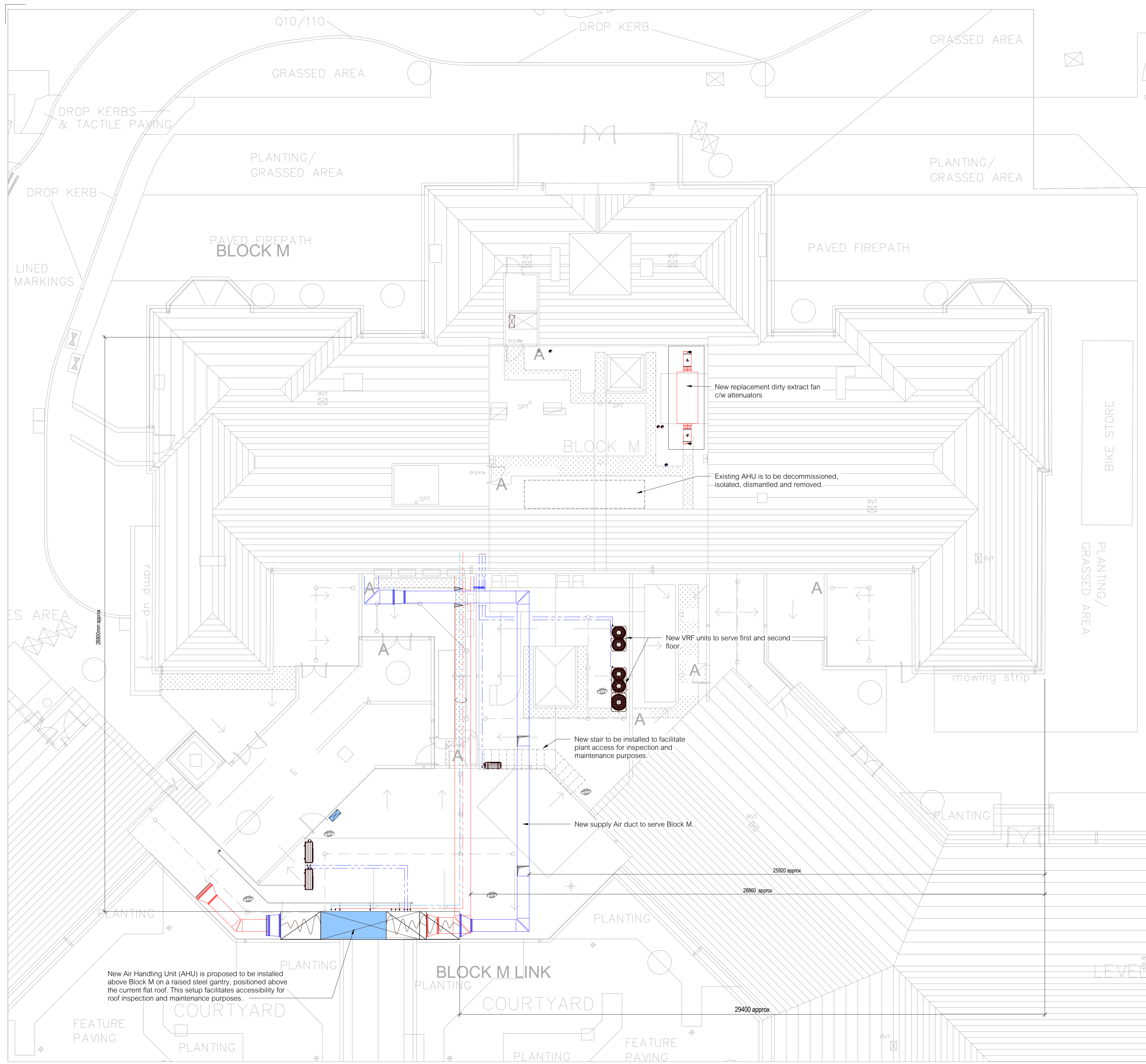
01 Roof Plan Proposed 1:100
