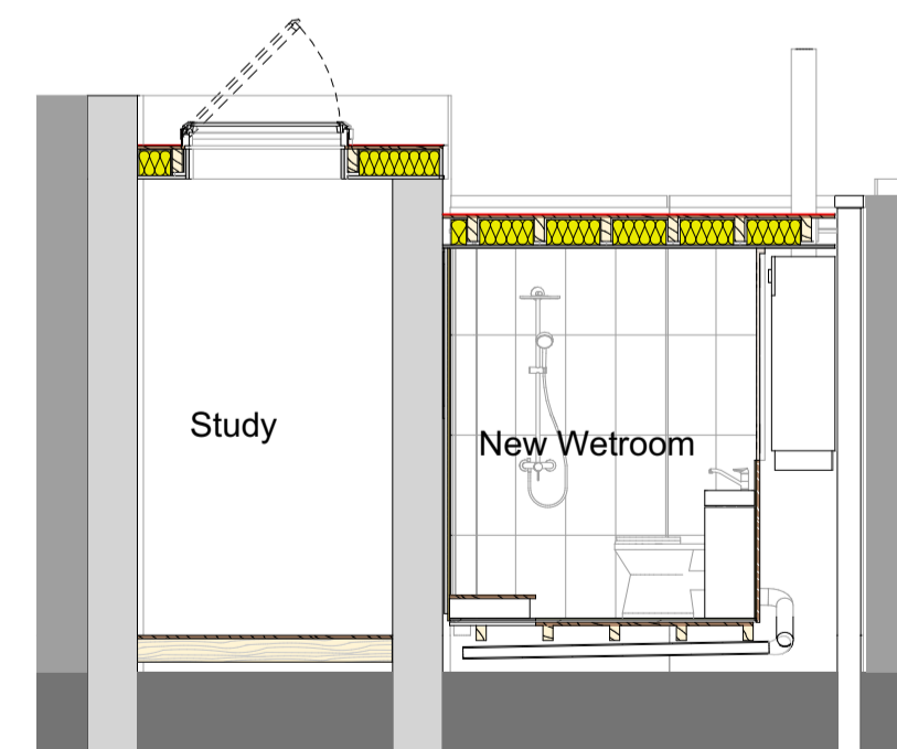
4 Proposed Cross Section 3 SCALE 1:50
