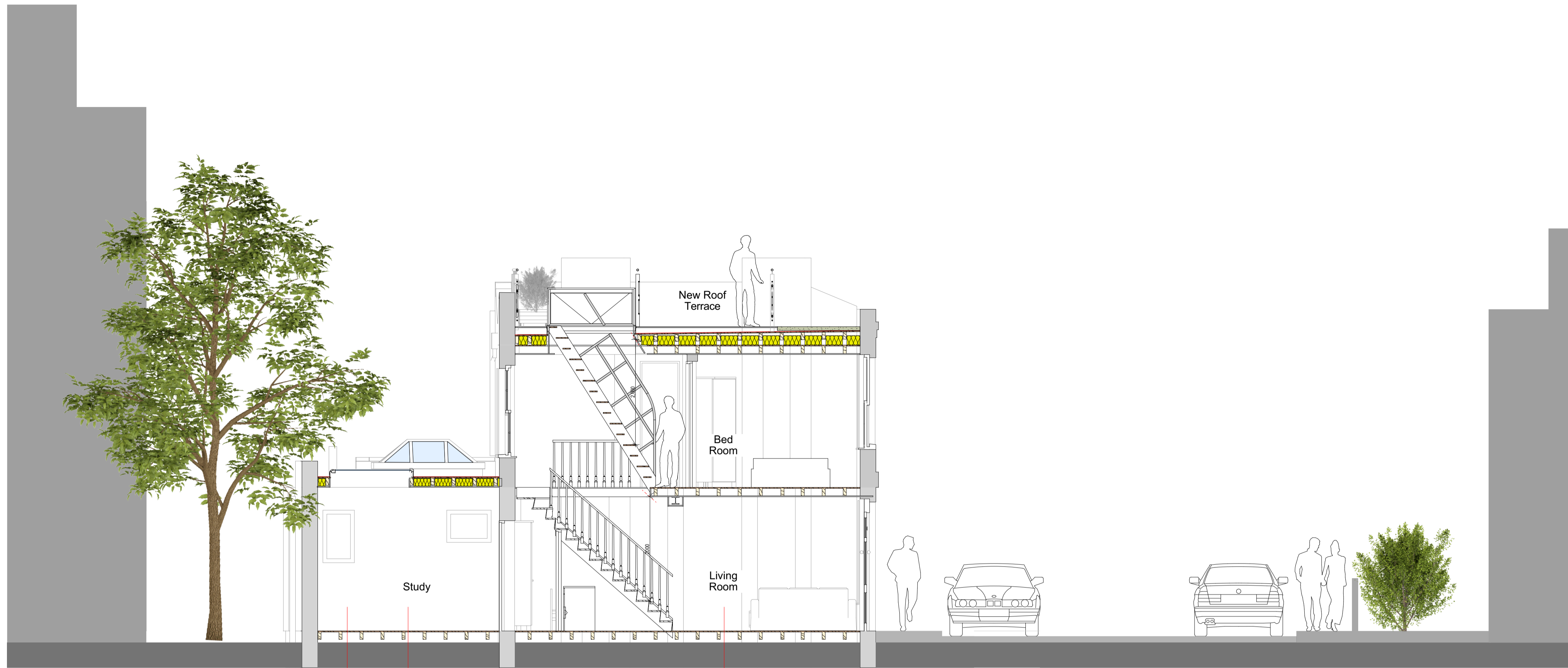
1 Proposed Long Section 1 SCALE 1:50
