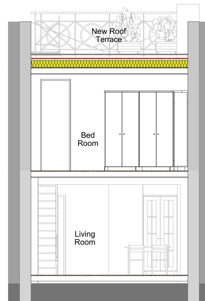
2 Proposed Cross Section 1 SCALE 1:50
