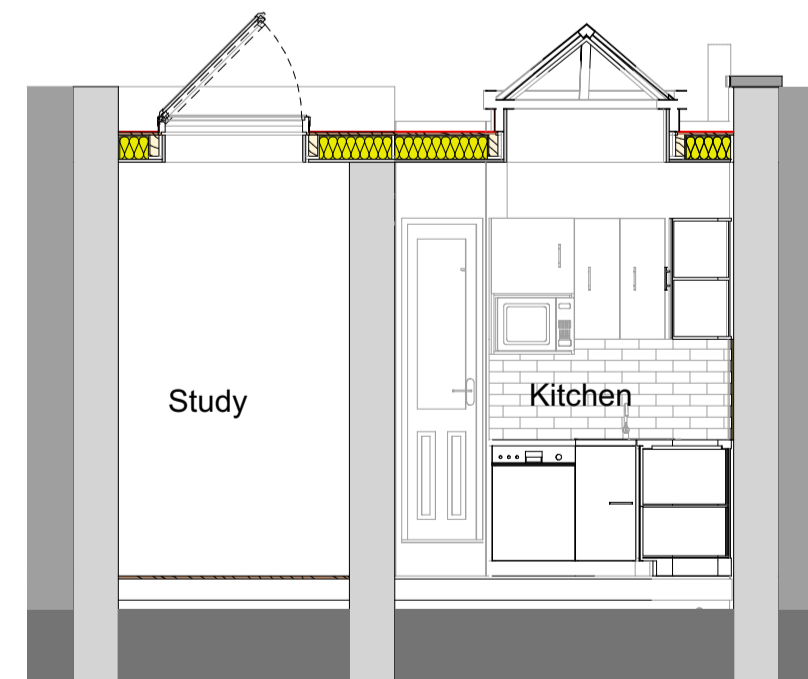
3 Proposed Cross Section 2 SCALE 1:50
