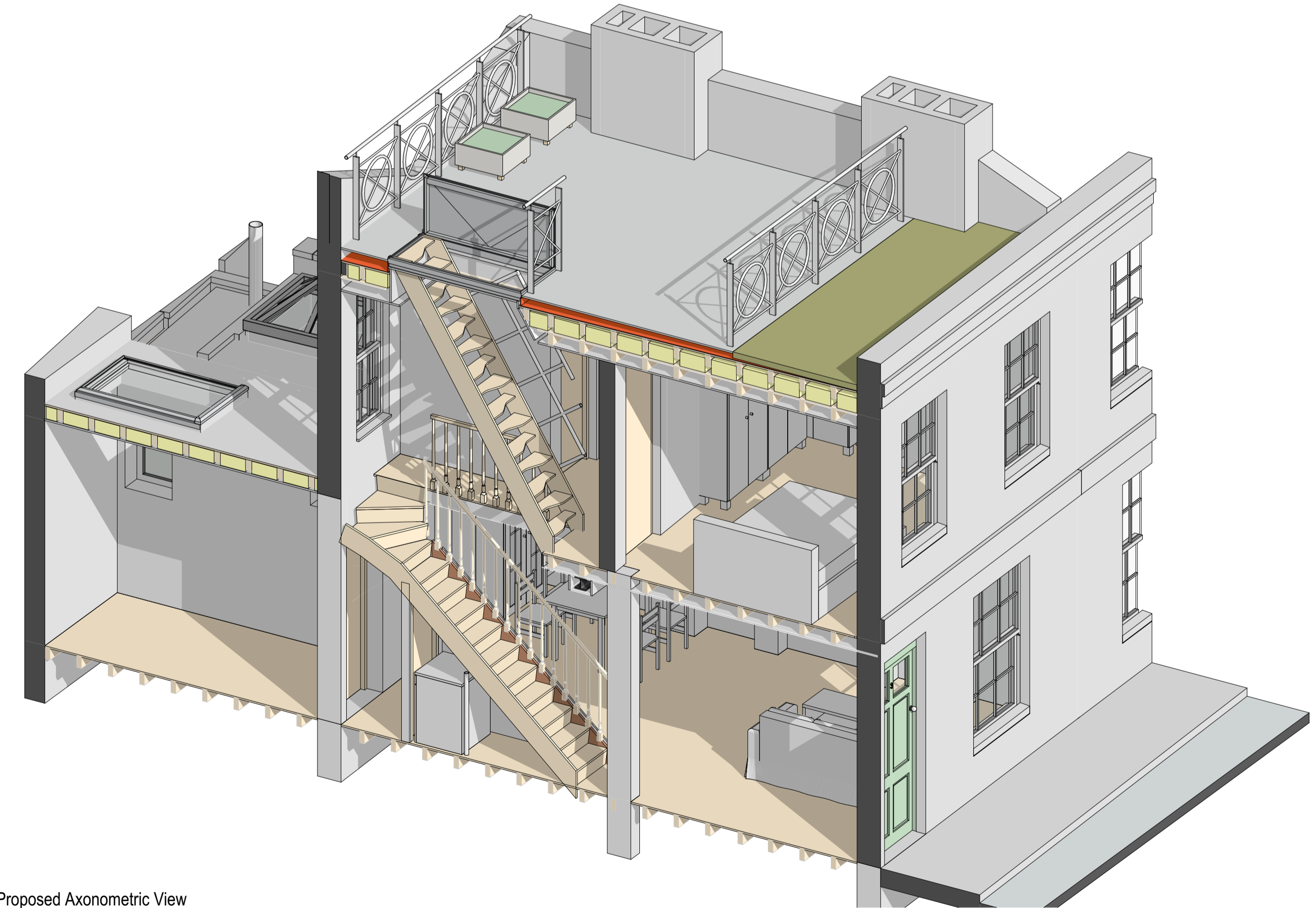
5 Proposed Axonometric View
