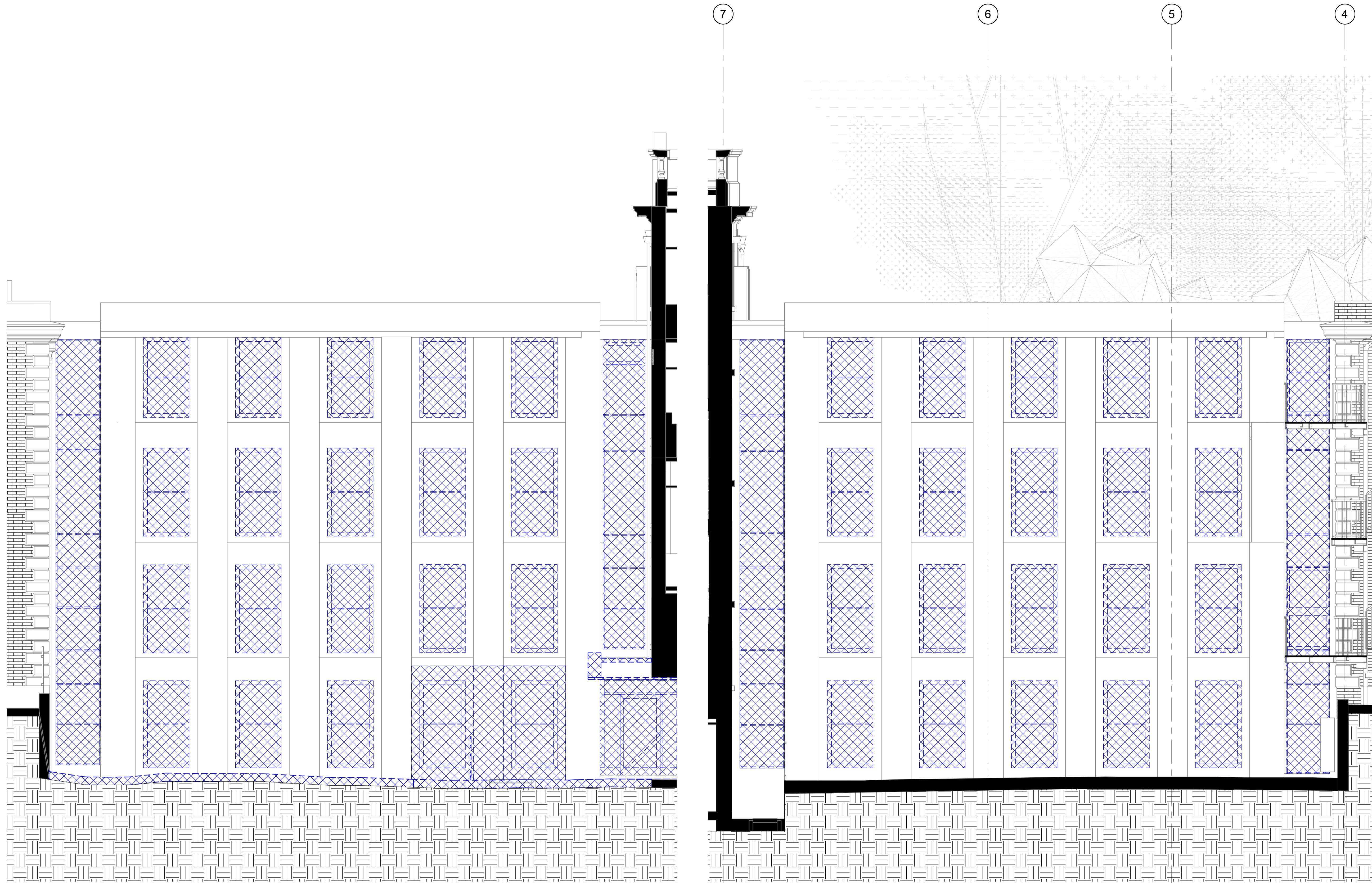
Demolition SW Elevation 1:50
