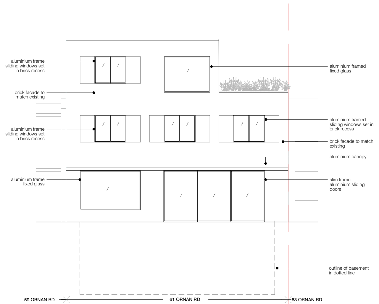
02 PROPOSED REAR ELEVATION scale 1:100
