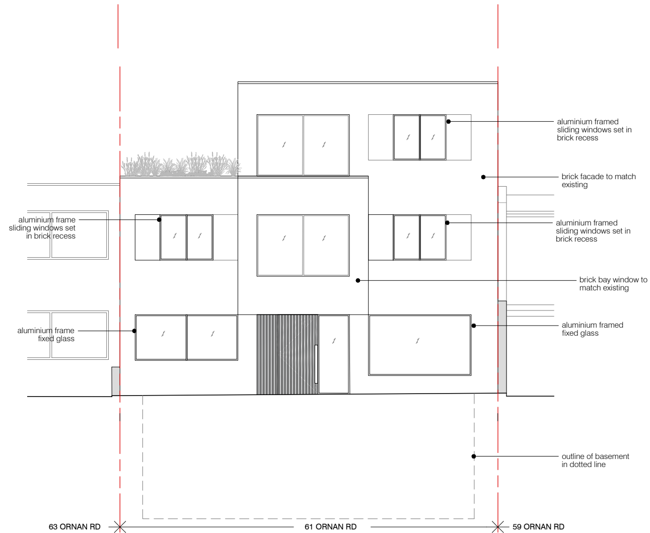
01 PROPOSED FRONT ELEVATION scale 1:100
