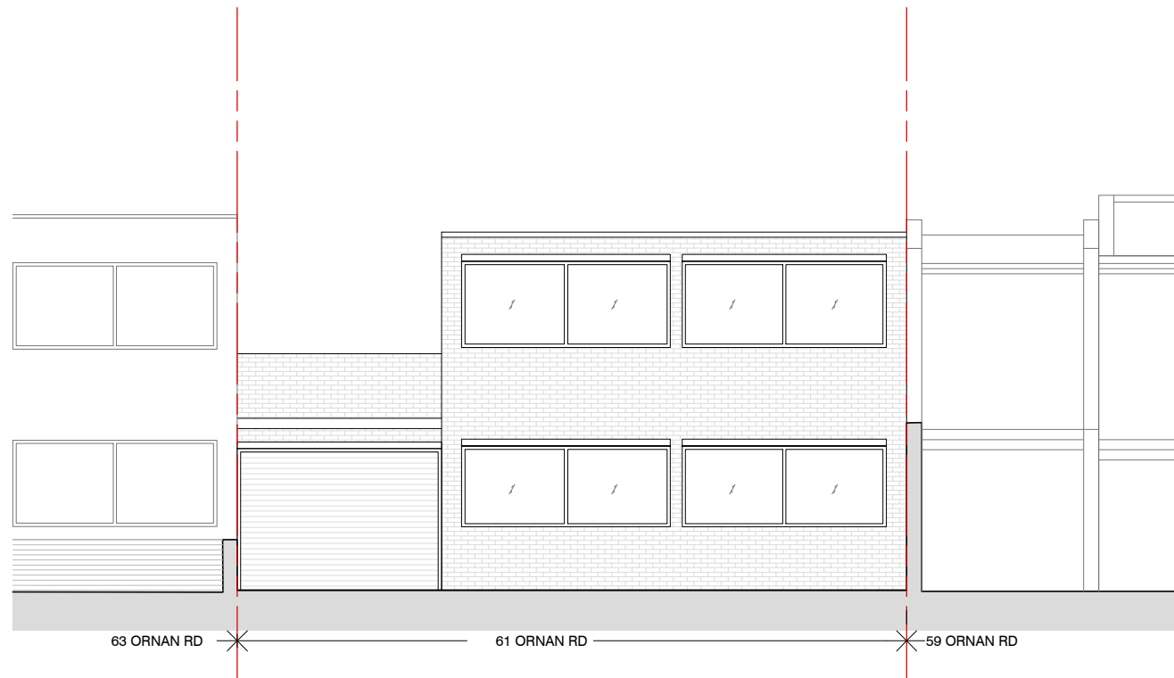
01 EXISTING FRONT ELEVATION scale 1:100
