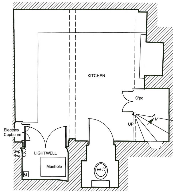
01 Existing Basement Plan 1:50@A3
