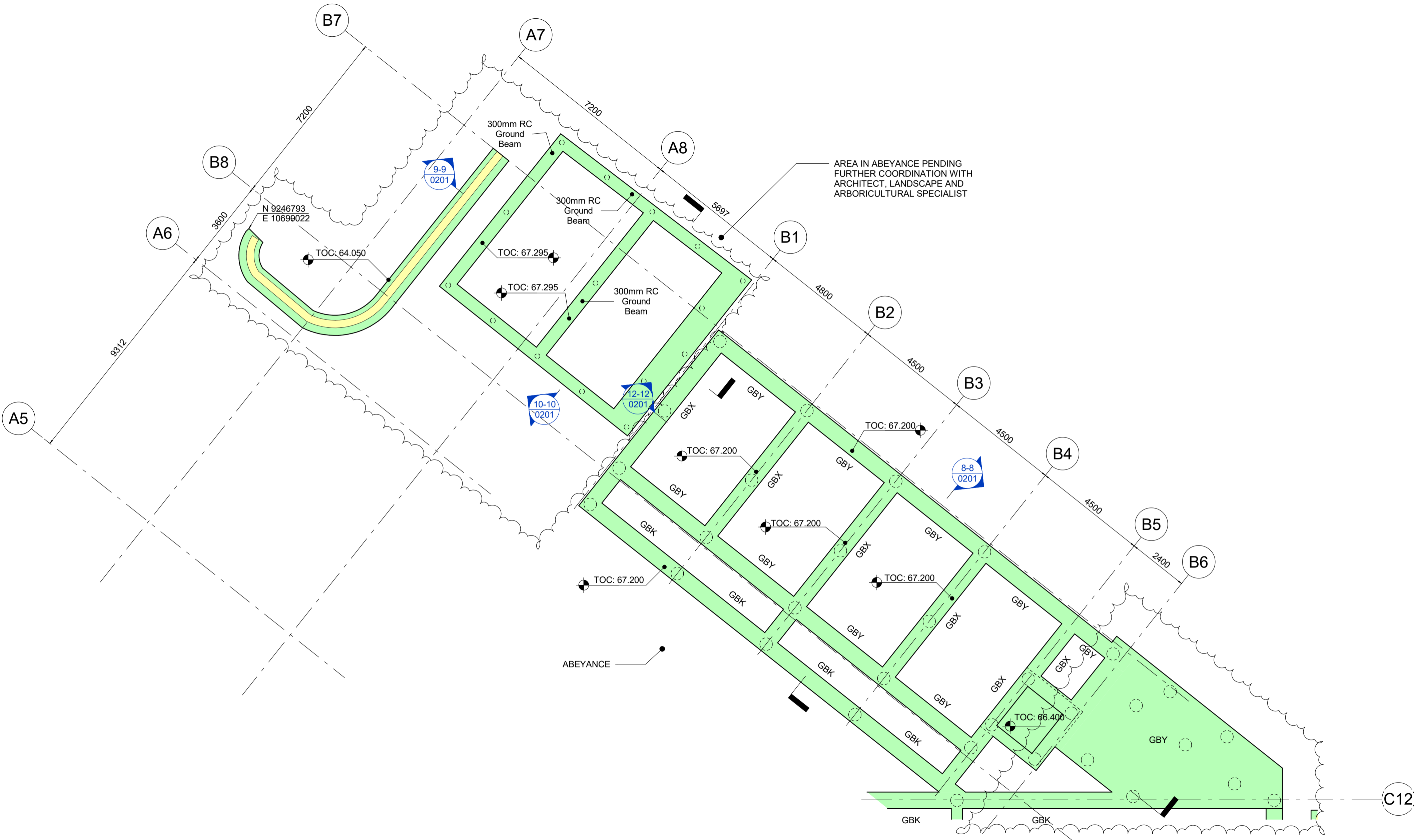
Block B Ground Floor - Foundations Layout
