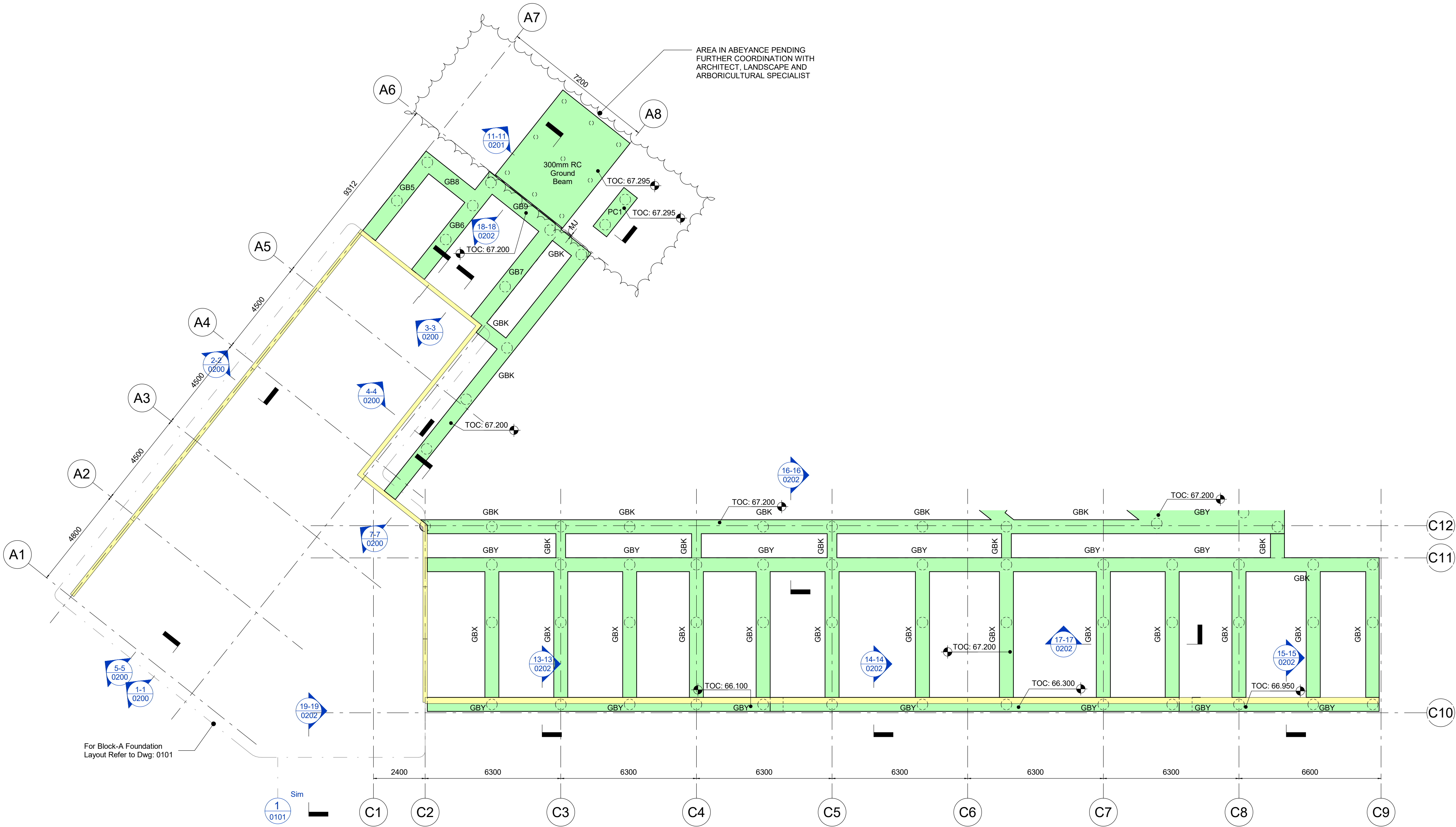
Block A & C Ground Floor - Foundations Layout
