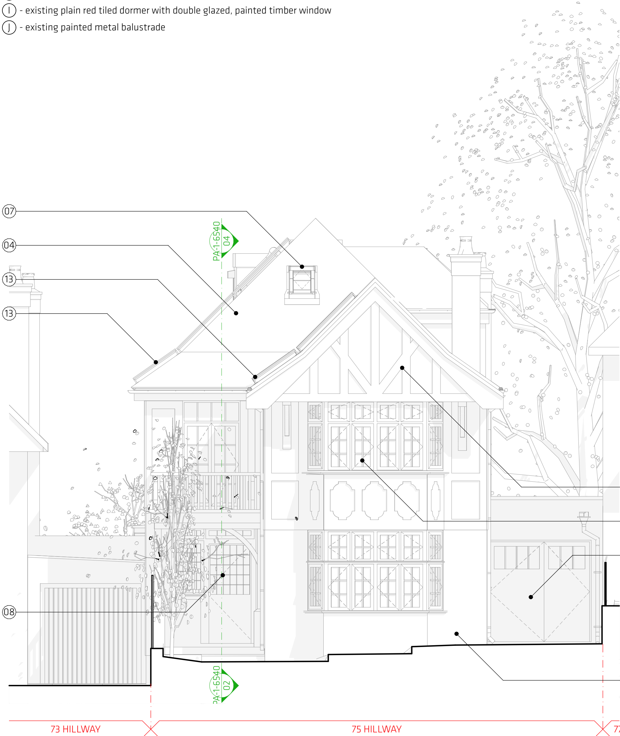
Proposed Elevation Front [NE] Scale @ A1: 1:50
