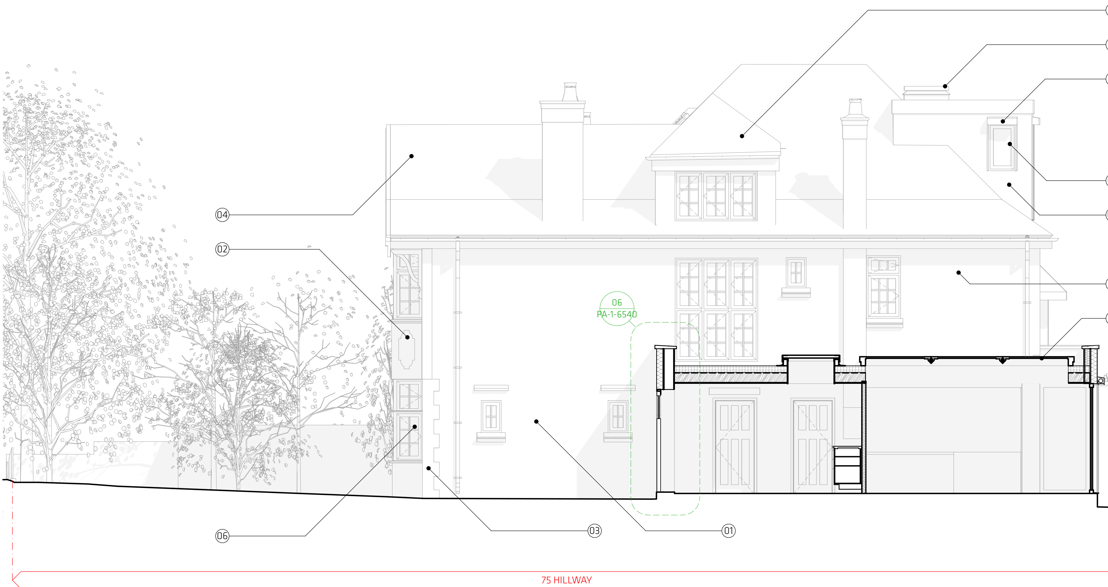
Proposed Elevation Side [NW] Scale @ A1: 1:50
