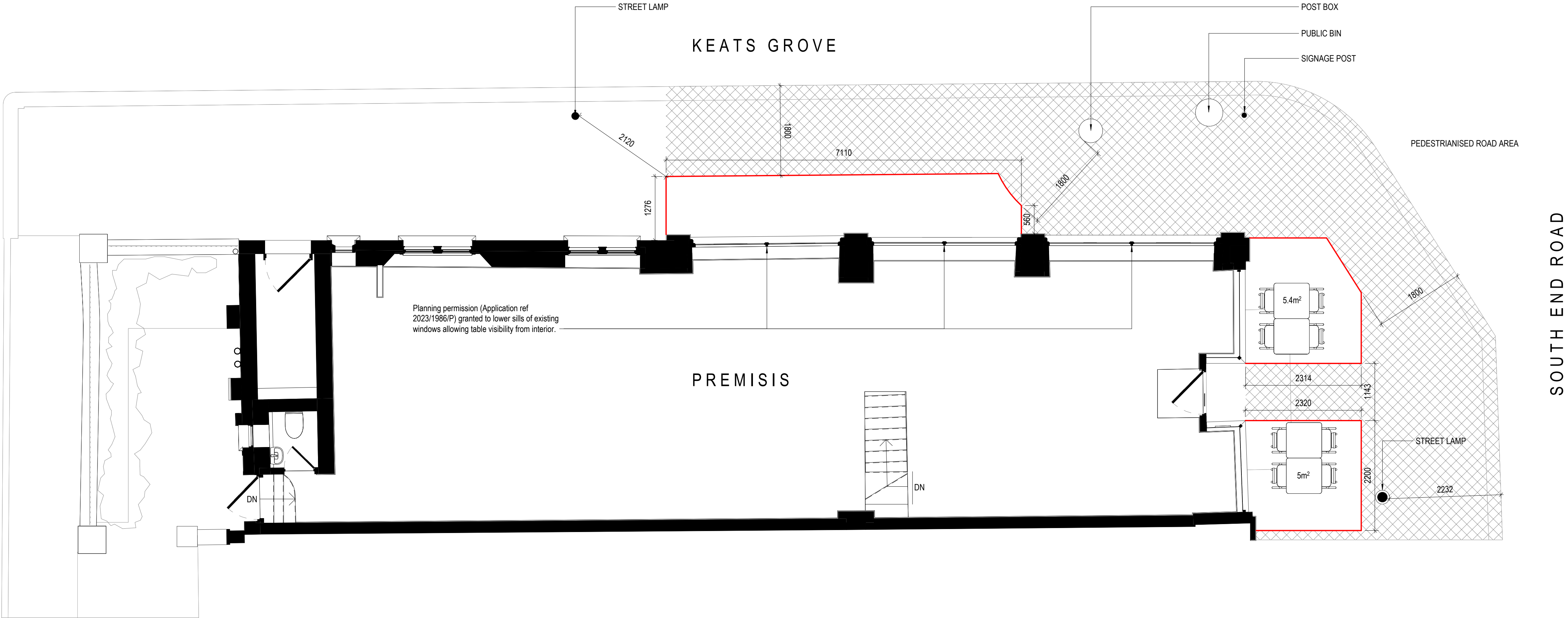
1 NEW 00 PLAN TABLES AND CHAIRS 1 : 50 @ A1
