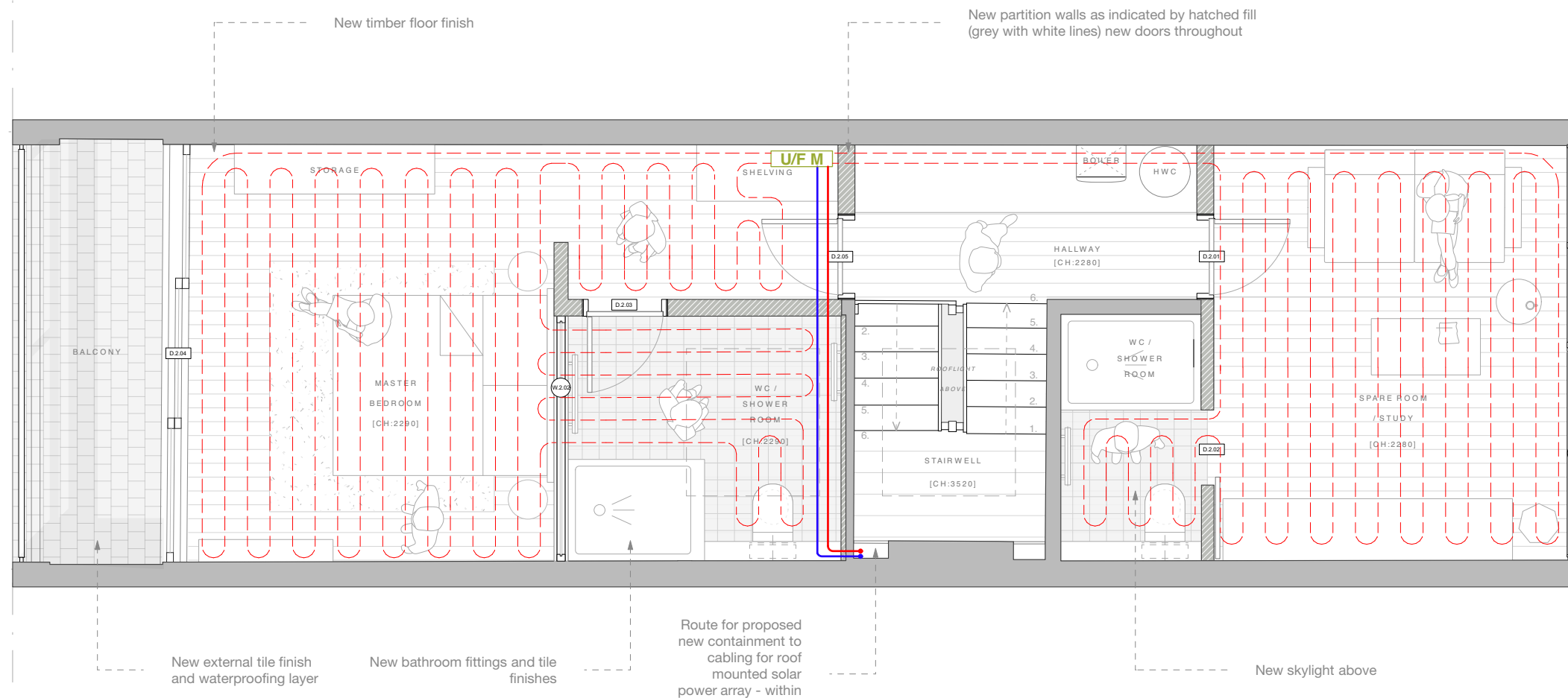
Second Floor Plan As Proposed 1:50 UFH Layout
