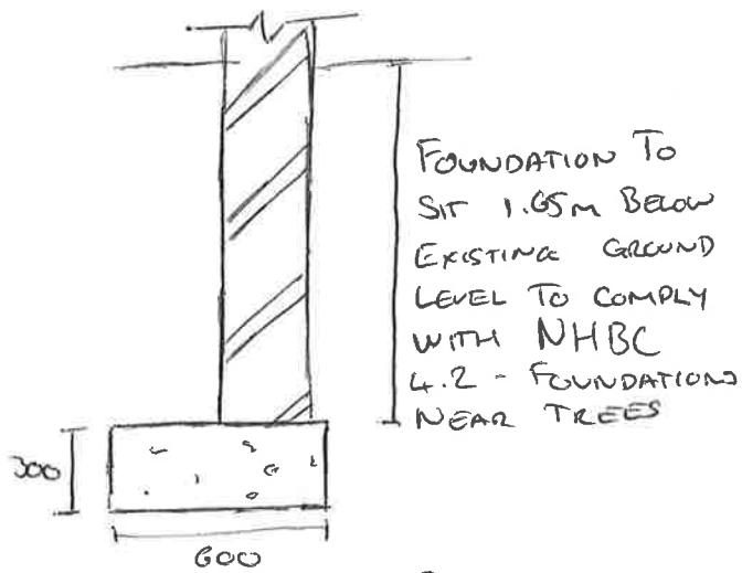
CROSS SECTION OF REAR WALL FOUNDATION BASE
